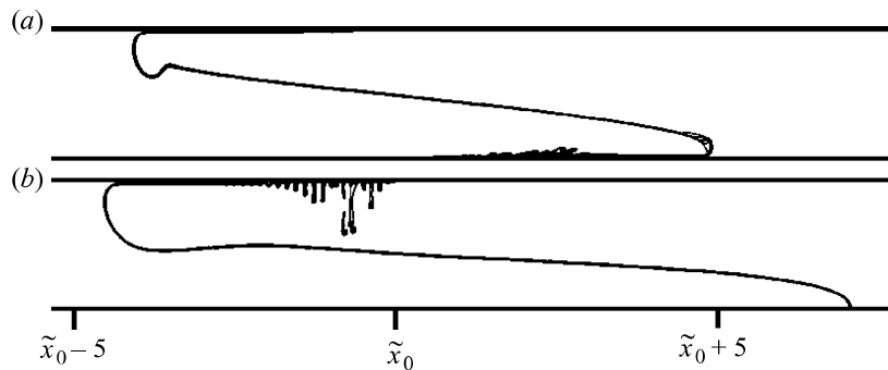
FIGURE 18. Iso-contours of \tilde{\rho} at \tilde{t} = 12.7 ( \rho_L/\rho_H = 10^{-3} , Re = 224 ) for (a) \mu_H = \mu_L and (b) \nu_H = \nu_L . Values of plotted iso-contours are \tilde{\rho} = 0.05 - 0.275 - 0.5 - 0.725 - 0.95 .
