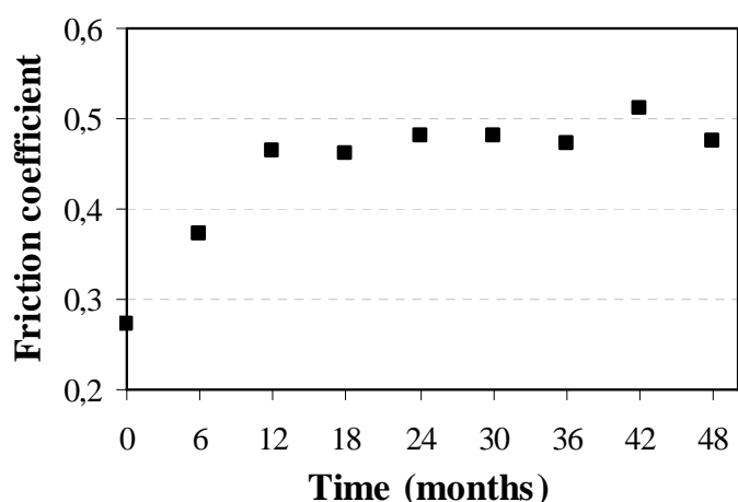
1 2 FIGURE 4 Evolution of friction coefficient due to natural ageing.
