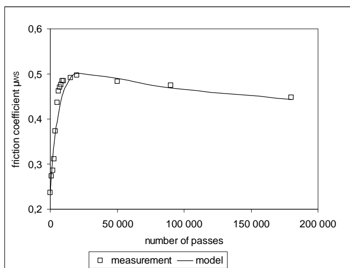
5 6 FIGURE 10 Comparison between Wehner/Schulze polishing curve and theoretical 7 predictions.
