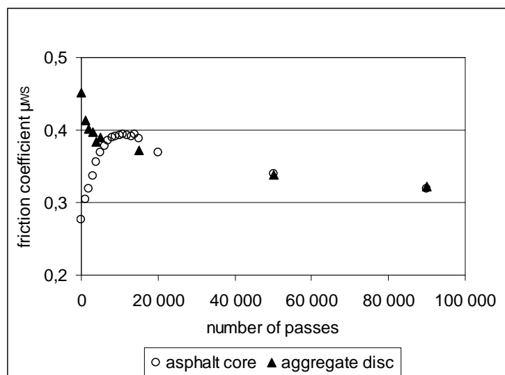
4 FIGURE 3 Friction evolution plot resulting from Wehner/Schulze polishing test.
