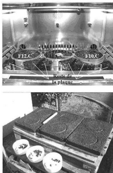
17 a) 18 FIGURE 5 Ageing test (a: weatherometer for accelerated test; b: specimens artificially 19 and naturally aged).
