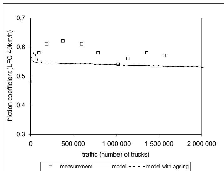
29 30 FIGURE 11 Comparison prediction/measurement of skid-resistance evolutions. 31
