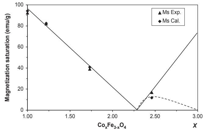
Fig. 4. Saturation magnetization ( M_S ) of \text{Co}_x\text{Fe}_{3-x}\text{O}_4 ( x=1.00, 1.22, 1.73, and 2.46 ) quenched at 900 °C, measured at 5 K and calculated at 0 K. The Néel model (solid line) is compared to the experimental results of Takahashi and Fine [13] (dashed line).
