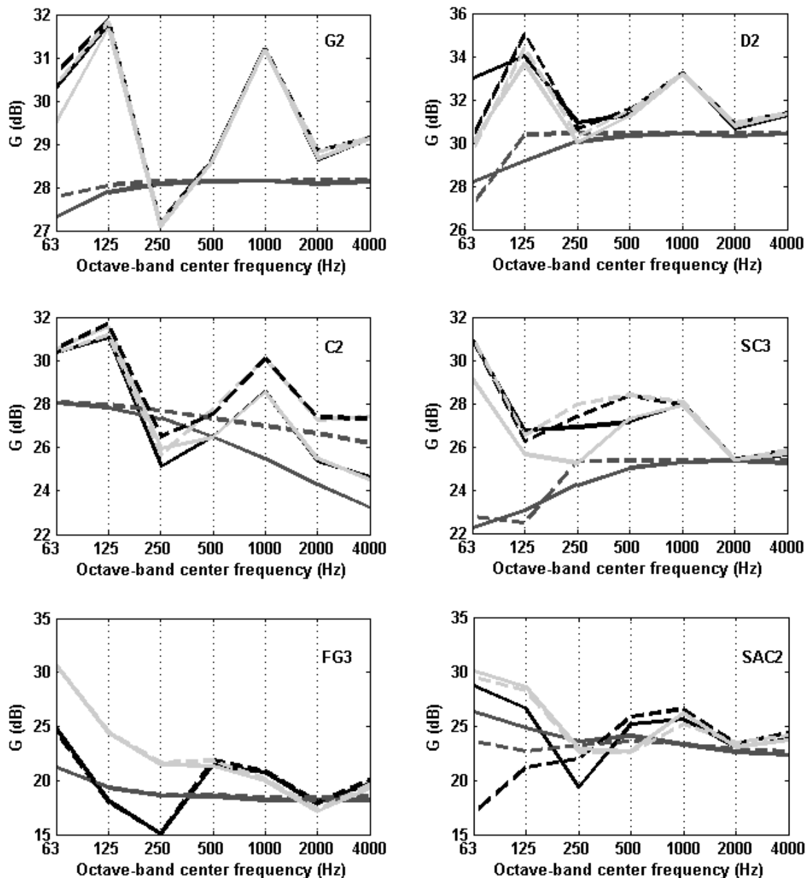
Figure 1: Predicted octave-band sound strength, G , for configurations G2, D2, C2, SC3, FG3 and SAC2. Solid lines: extended reaction; dashed lines: local reaction. Black lines: WBC; light grey lines: WBR, dark grey lines: EBR.
