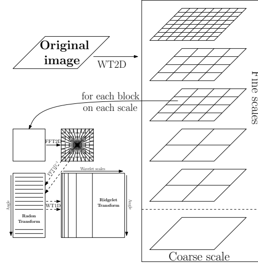
Figure 2: Scheme showing the main steps of the curvelet-99 transform : the ridgelet transform is applied to each block of each scale of an isotropic 2D wavelet transform.
