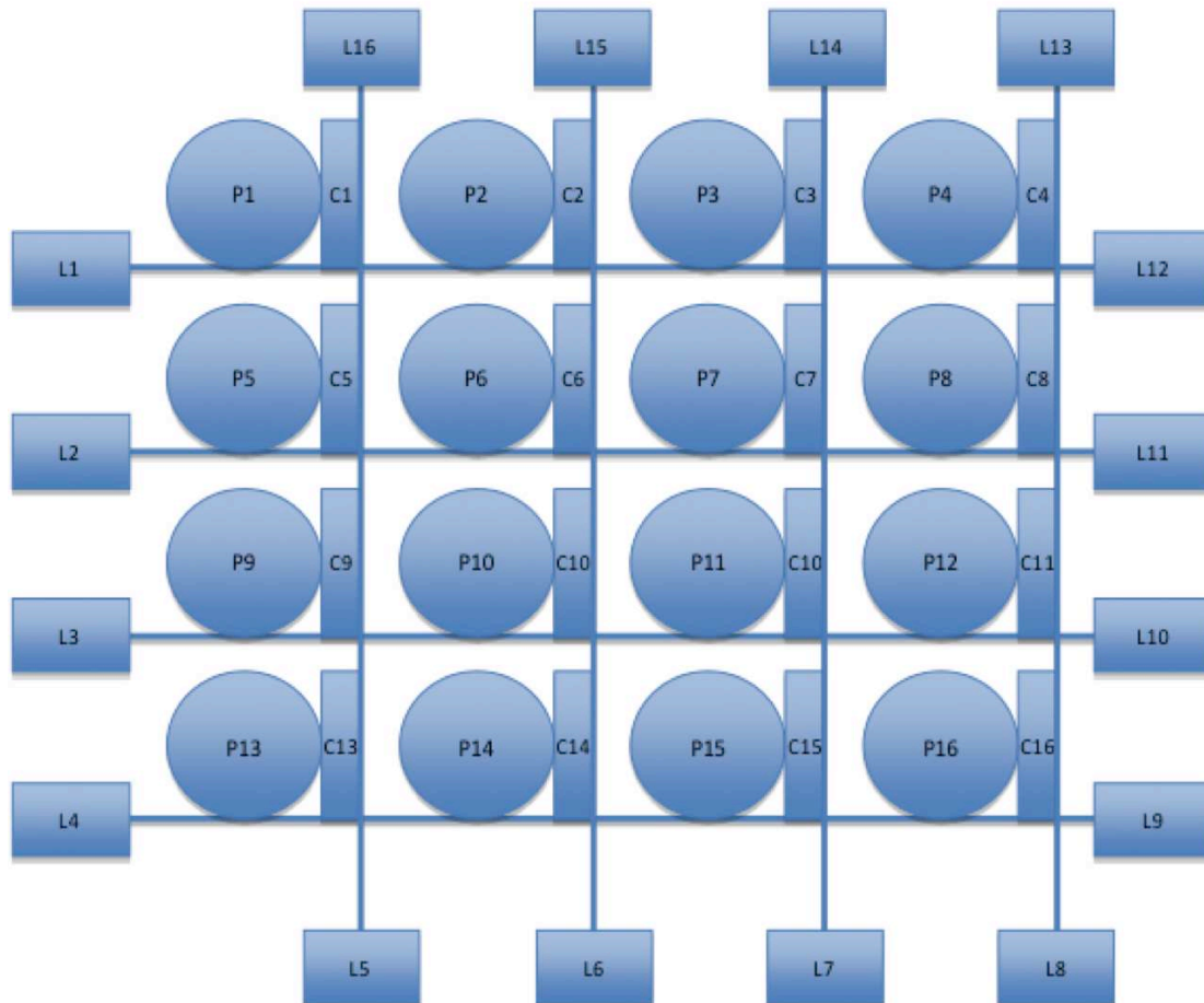
Figure 2: Illustration of an imaging system in CMOS 0.35 \mu\text{m} Opto. An example of 4x4 photodiodes matrix, each photodiode has its read-out circuit.
