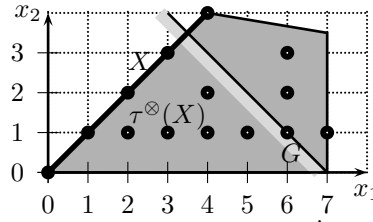
Figure 2: Finite-cardinality translation: \tau : x_1 + x_2 \leq 7 \rightarrow x'_1 = x_1 + x_2 \wedge x'_2 = x_2 with X_0 = (0 \leq x_1 = x_2 \leq 4) : reachable points and polyhedron computed by abstract acceleration (see §4.4).
