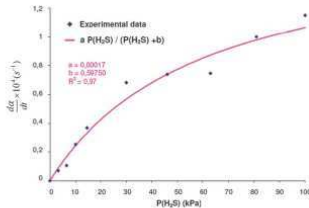
Figure 17 : Variation of the reaction rate versus P(H_2S) of ZnO sulfidation for the same fractional conversion ( \alpha=0.3 ) at 260^\circ\text{C} , P(H_2S) variable up to 100 kPa, P(H_2O)=1.8 kPa.
