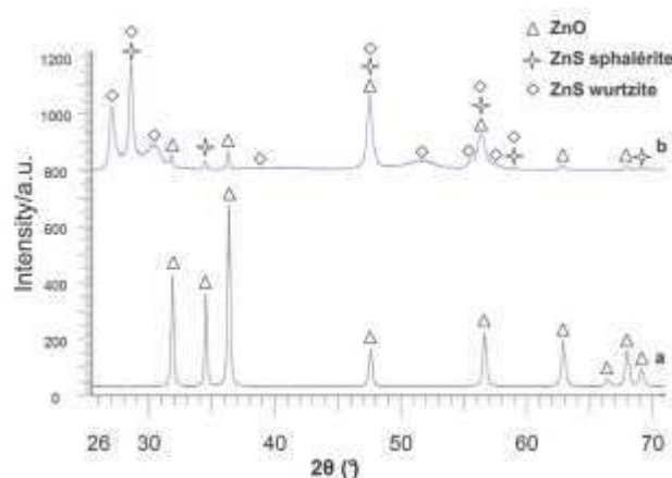
Figure 8 : XRD patterns obtained for (a) ZnO sample before sulfidation, (b) ZnO sample after sulfidation at 310^\circ\text{C} , P(\text{H}_2\text{S})=5 kPa and P(\text{H}_2\text{O})=2.5 kPa ( \alpha=0.9 ).
