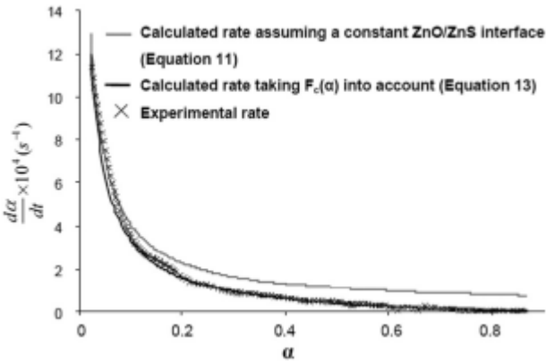
Figure 20 : Comparison between experimental and calculated reaction rates for ZnO sulfidation at 310°C, P(\text{H}_2\text{S})=5 \text{ kPa} and P(\text{H}_2\text{O})=2.5 \text{ kPa} . The calculated rates were determined assuming a constant ZnO–ZnS internal interface (grey line) and by taking F_c(\alpha) into account (black line).
