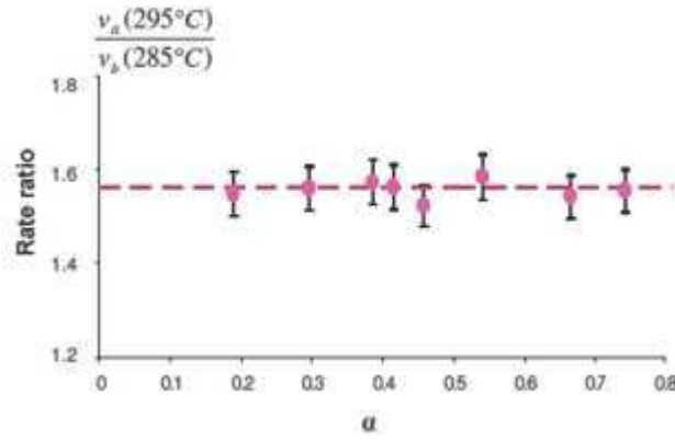
Figure 11 : Ratios of the rates after and before the jumps from 285 to 295°C as a function of \alpha , P(\text{H}_2\text{S})=5 kPa.
