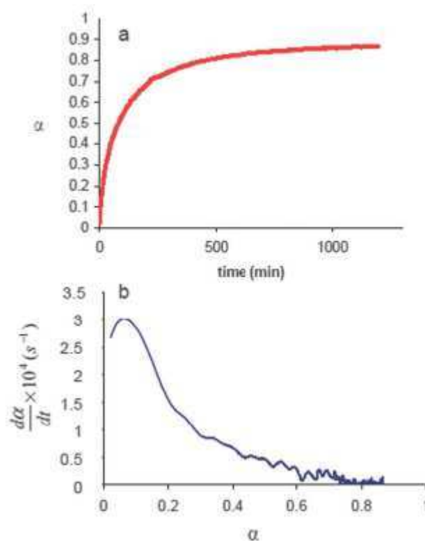
Figure 1 : (a) variation of the fractionnal conversion versus time of ZnO sulfidation at 310°C, P(H 2 S)=5kPa and P(H 2 O)=2,5kPa. (b) variation of the reaction rate d\alpha/dt as a function of fractionnal conversion \alpha .
