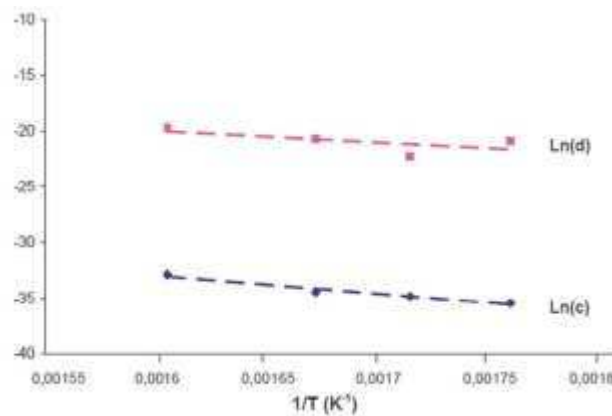
Figure 18 : Representation of Ln(c) and Ln(d) functions of 1/T for ZnO sulfidation reaction at various temperatures 295–310–325–350°C, P(H 2 S)=5 kPa, P(H 2 O)=2.5 kPa, where c and d are the values expressed in eqn (14).
