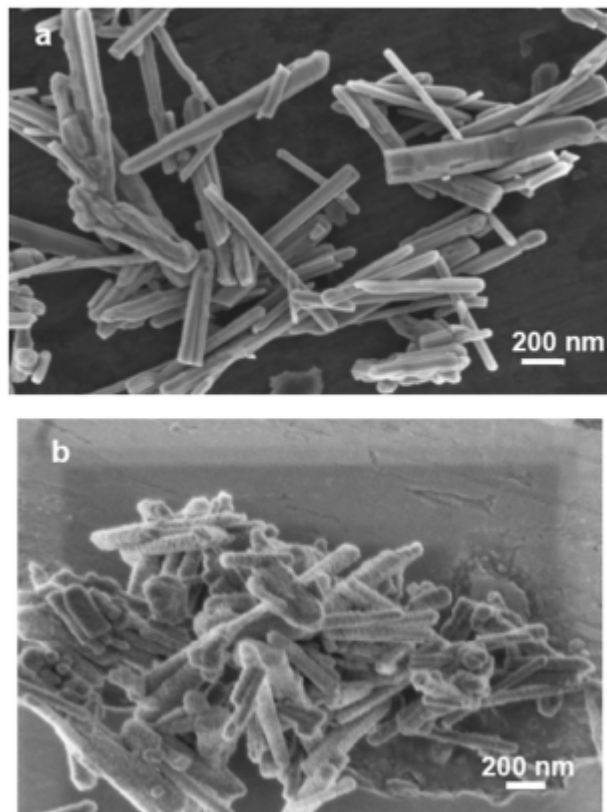
Figure 13 : SEM micrographs of ZnO particles: (a) before sulfidation and (b) after sulfidation at 295°C and P(\text{H}_2\text{S})=10 kPa at very low fractional conversion ( \alpha \approx 0.01 ).
