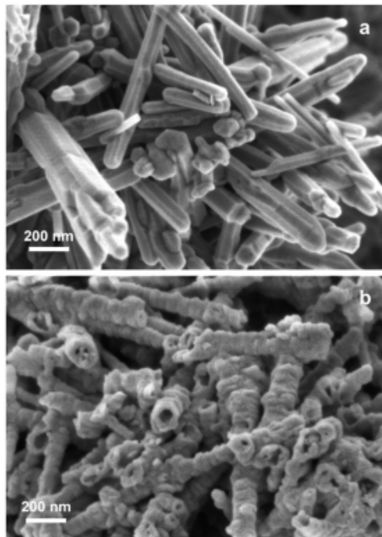
Figure 3: SEM micrographs of ZnO particles: (a) before sulfidation and (b) after sulfidation at 295°C and P(H 2 S)=10 kPa ( \alpha=0.9 )
