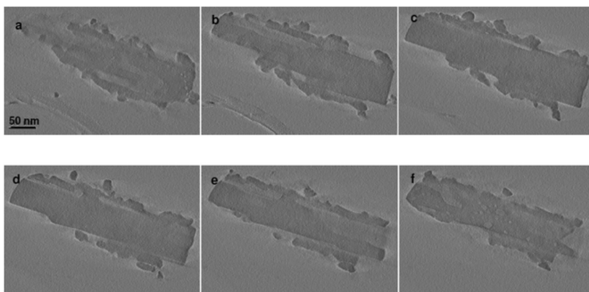
Figure 6 : Electron tomography study of a partially sulfided ZnO particle ( \alpha=0.3 ) at 230°C, P(\text{H}_2\text{S})=5 kPa and P(\text{H}_2\text{O})=2.5 kPa (from a to f). Numerical slices (0.55 nm thickness) of the 3D reconstruction in a perpendicular plane to the electron beam from the upper rod surface to the lower rod surface.
