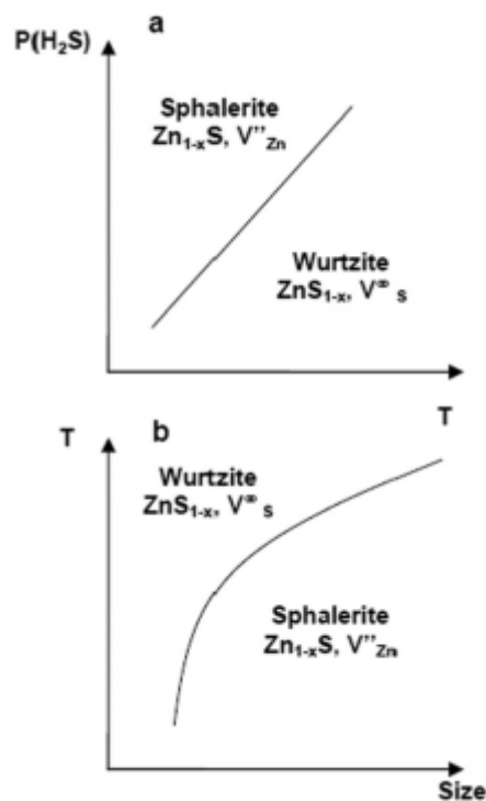
Figure 10 : Schematic representations of ZnS sphalerite–wurtzite phase transition, (a) 36–38 as a function of temperature and P(\text{H}_2\text{S}) , (b) 40 as a function of temperature and ZnS crystal size.
