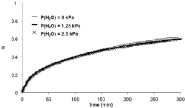
Figure 16 : Variation of the fractional conversion versus time of ZnO sulfidation at 295^\circ\text{C} , P(\text{H}_2\text{S})=5 kPa and various P(\text{H}_2\text{O}) .
