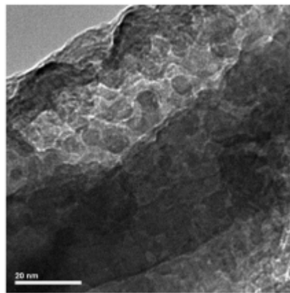
Figure 7: TEM micrograph of a partially sulfided ZnO particle ( \alpha=0.3 ) at 230^\circ\text{C} , P(\text{H}_2\text{S})=5 kPa and P(\text{H}_2\text{O})=2.5 kPa.
