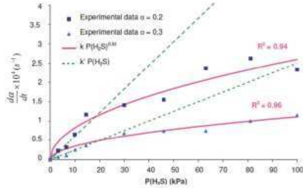
Figure 14 : Variation of the kinetic rate versus P(\text{H}_2\text{S}) of ZnO sulfidation for the same fractional conversion ( \alpha=0.2 and \alpha=0.3 ) at 260°C, P(\text{H}_2\text{S}) variable up to 100 kPa, P(\text{H}_2\text{O})=1.8 kPa.
