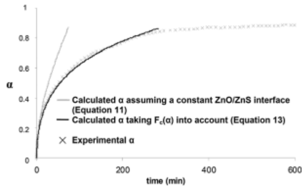
Figure 21 : Comparison between the experimental and calculated fractional conversions (from eqn (11) and (13)) for ZnO sulfidation at 310°C, P(\text{H}_2\text{S})=5 kPa and P(\text{H}_2\text{O})=2.5 kPa.
