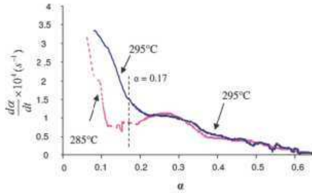
Figure 12 : Sudden temperature change from 285 to 295°C at \alpha=0.17 and comparison to the experiment done at 295°C, P(\text{H}_2\text{S})=5 kPa.
