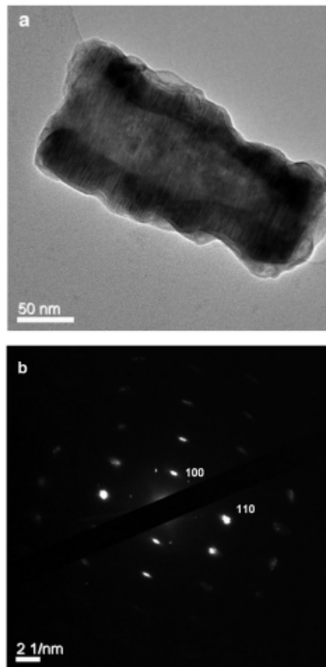
Figure 9 : (a) TEM micrograph of almost totally sulfided ZnO ( \alpha=0.9 ) at 295°C, P(\text{H}_2\text{S})=5 kPa. (b) Selected-area electron diffraction pattern of the whole particle.
