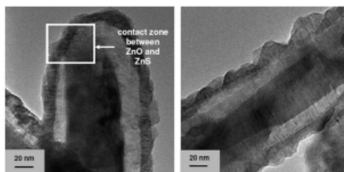
Figure 4: TEM micrographs of partially sulfided ZnO particles ( \alpha=0.3 ) at 230°C, P(H 2 S)=5 kPa and P(H 2 O)=2.5 kPa
