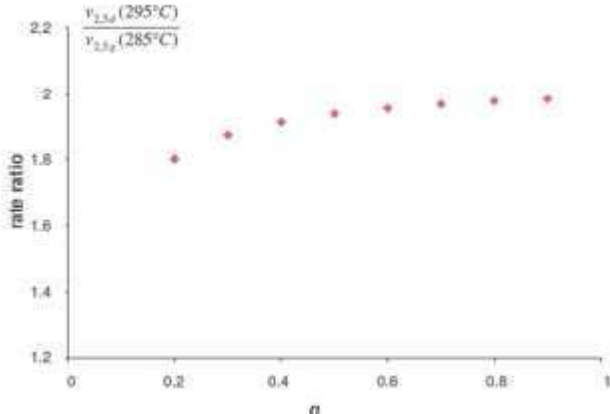
Figure 19 : Calculated rate ratios after and before the jumps from 285 to 295°C functions of \alpha , P(\text{H}_2\text{S})=5 \text{ kPa} , P(\text{H}_2\text{O})=2.5 \text{ kPa} .
