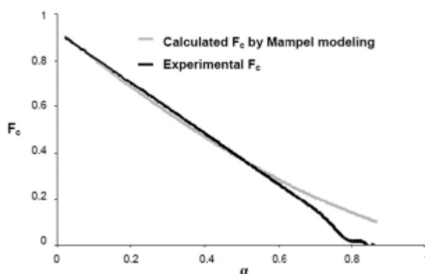
Figure 22 : Evolution of the calculated ZnO–ZnS interface surface fraction F_c(\alpha) obtained by Mampel modeling and the experimental surface fraction F_c(\alpha) obtained from the experimental and calculated rate curves for ZnO sulfidation at 310°C, P(\text{H}_2\text{S})=5 kPa and P(\text{H}_2\text{O})=2.5 kPa.
