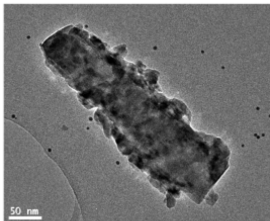
Figure 5 : TEM micrograph at 0° tilt angle of a partially sulfided ZnO particle ( \alpha=0.3 ) at 230°C, P(\text{H}_2\text{S})=5 kPa and P(\text{H}_2\text{O})=2.5 kPa. Gold nanoparticles (black dots) are used as fiducial markers for tilt series alignment.
