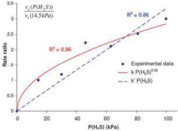
Figure 15 : Ratios of the kinetic rates after and before the jumps from a \text{H}_2\text{S} partial pressure of 14.5 kPa to various \text{H}_2\text{S} partial pressures as a function of P(\text{H}_2\text{S}) at 260^\circ\text{C} , P(\text{H}_2\text{O})=1.8 kPa, \alpha=0.34 .
