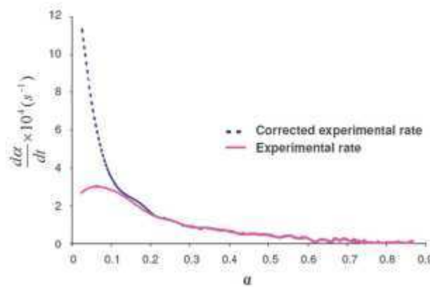
Figure 2 : Correction of the experimental reaction rate of ZnO sulfidation at 310^\circ\text{C} , P(H_2S)=5\text{kPa} and P(H_2O)=2,5\text{kPa} .
