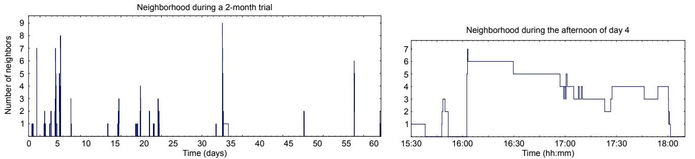
Figure 4: Evolution of the neighborhood of netbook n14 during the 2-month trial
