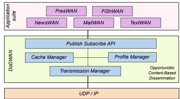
Figure 1: Architecture of the DoDWAN system
