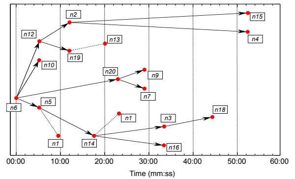
Figure 5: Timeline of the dissemination of a message
