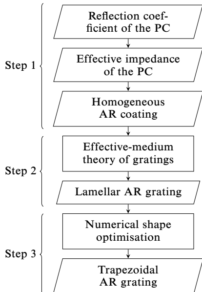
FIG. 3: Successive steps of the proposed AR grating design algorithm.
