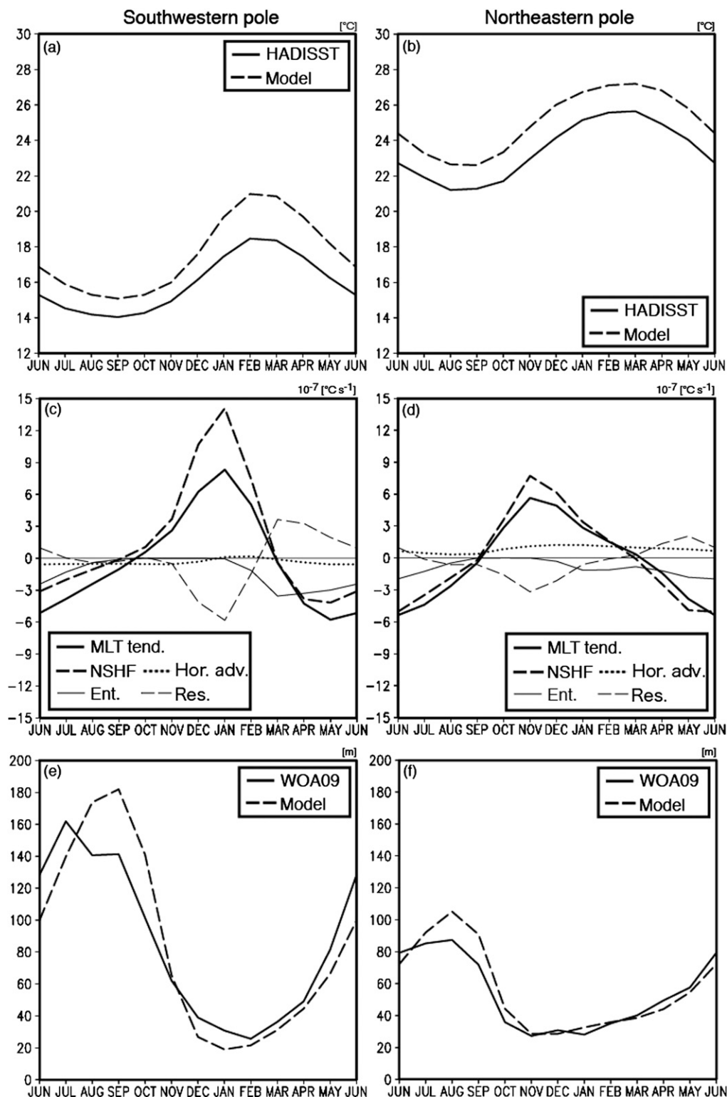
FIG. 3. Seasonal cycle of (a),(b) SST ( ^{\circ}\text{C} ), (c),(d) each term in Eq. (1) ( 10^{-7} \text{ } ^\circ\text{C s}^{-1} ), and (e),(f) mixed layer depth (m) at the southwestern and northeastern poles of the IOSD defined in Fig. 2b. In (a),(b) the SSTs from HADISST (solid line) and SINTEX-F model (dashed line) are shown. In (c),(d) the mixed layer temperature tendency (MLT tend., thick solid line), net surface heat flux (NSHF, thick dashed line), horizontal advection (Hor. adv., thick dotted line), entrainment (Ent., thin solid line) and residual (Res., thin dashed line) terms are shown. In (e),(f), the mixed layer depths derived from WOA09 (solid line) and the model (dashed line) are shown.
