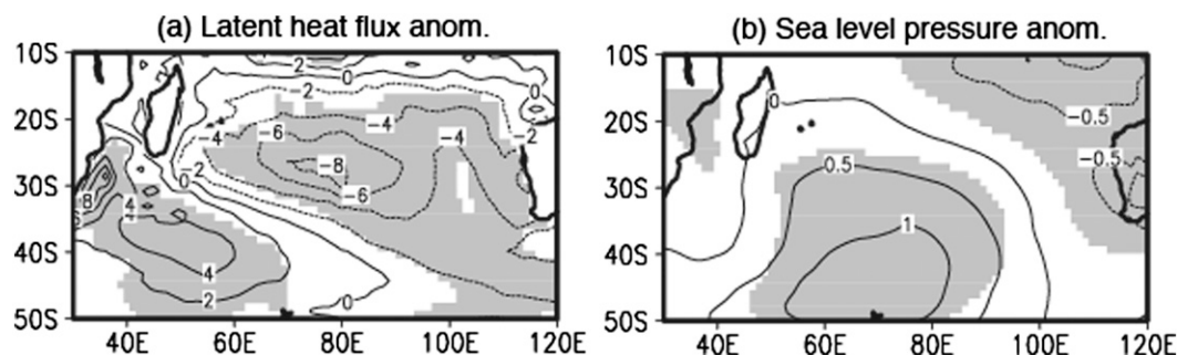
FIG. 11. Composite anomalies of (a) LH ( \text{W m}^{-2} ) and (b) SLP (hPa) averaged during November (0)–January (1) of the positive IOSD. The anomalies exceeding 99% confidence level by two-tailed t test are shaded.
