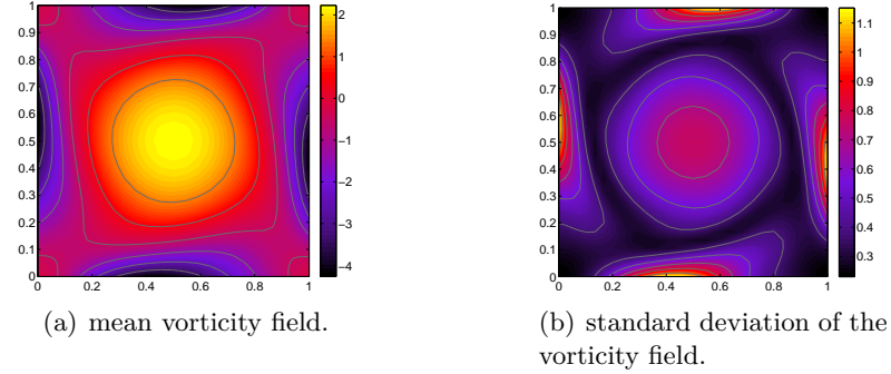
Figure 8: Rank-45 PGD approximation for Test 2.
