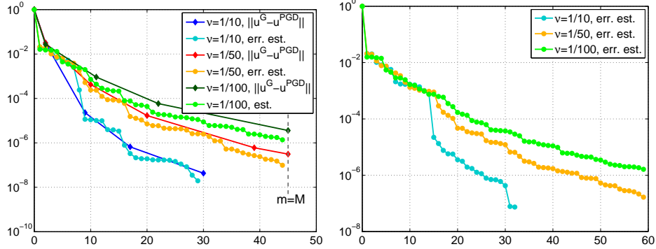
Figure 10: Test 2: convergence of error \epsilon(m) and of the relative norm of \lambda_m with respect to the rank ( m ) of the PGD approximation for \bar{\nu}' = 1/10, 1/50, 1/100 , considering N = 8 (left) and N = 15 (right) random variables.
