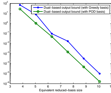
Figure 3: Mean of dual-based error bound, when using a POD or a Greedy basis selection procedure, for different reduced basis sizes.
