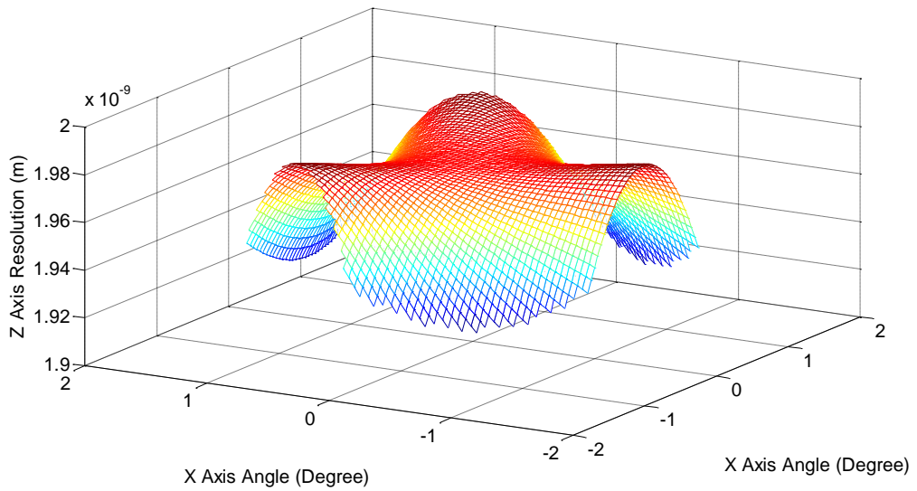
(b) Z=220um plane's resolution distribution
