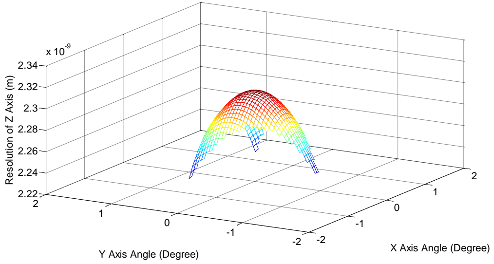
(a) Z=100um plane's resolution distribution
