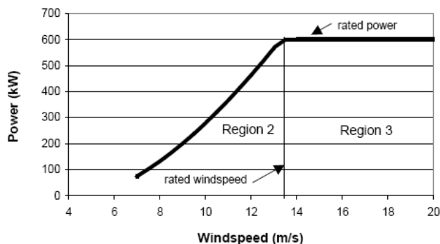
Fig.1 Typical wind turbine power curve
