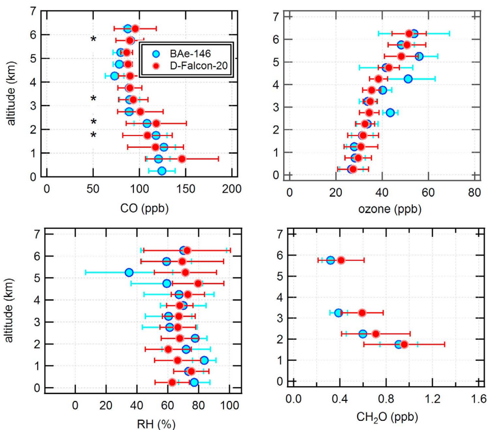
Figure 2. Comparison of the 3 physico-chemical tracers (CO, ozone and relative humidity, RH) and \text{CH}_2\text{O} from the BAe-146 and D-Falcon20 aircraft in zone 1. The stars mark the altitude bins where physico-chemical tracers are statistically comparable.
