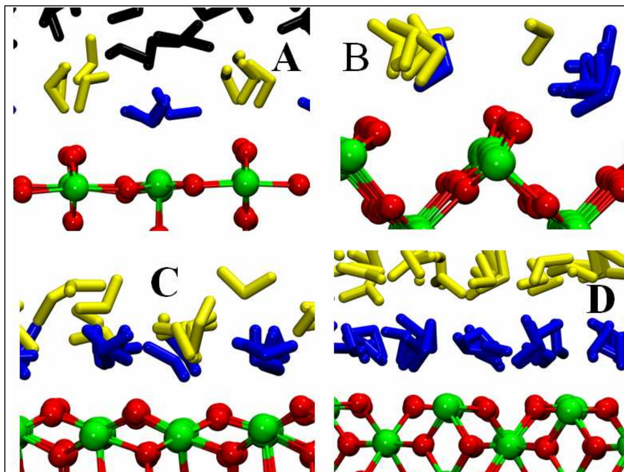
Fig. 1: Representative configurations of various rutile-water interfaces: (A) (110), (B) (100), (C) (010), and (D) (001). (blue- 1 ML, yellow- 2 ML)
