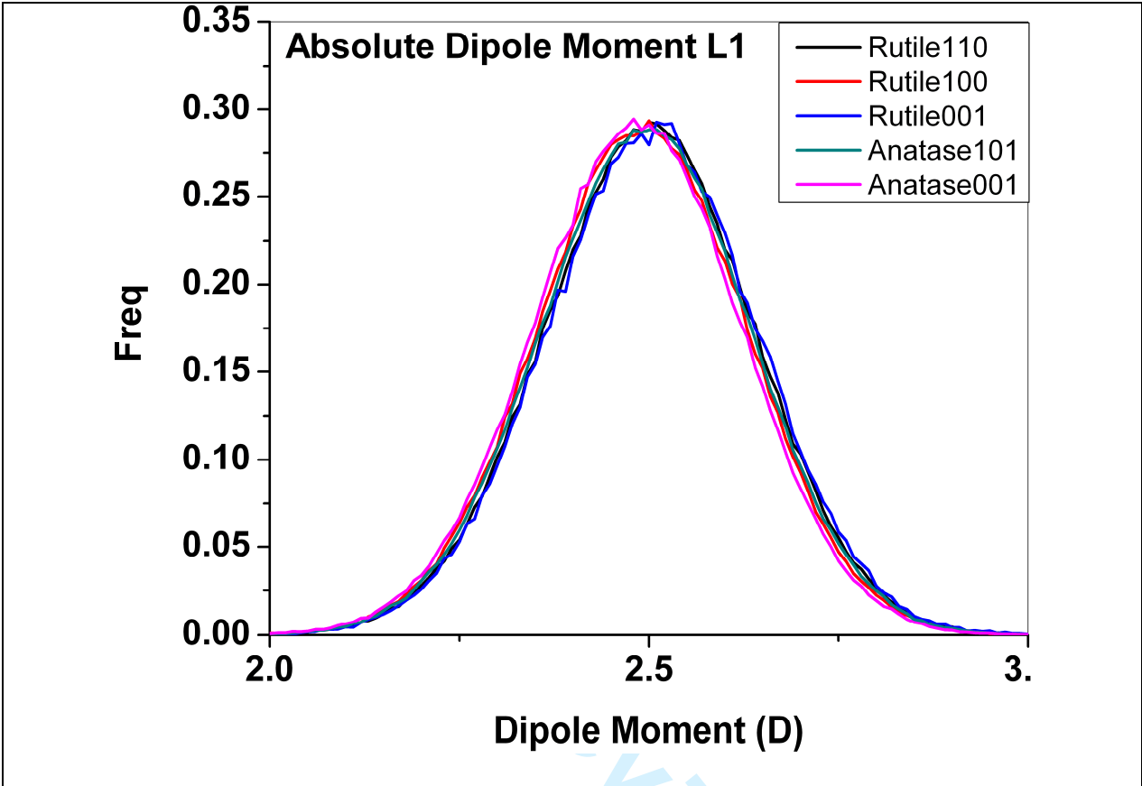
Fig. 6: Distribution of the water absolute dipole moment within 0 to 5 Å from the surface.
