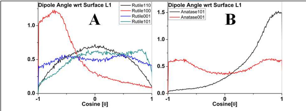
Fig. 7: Distribution of the cosine of angle of water molecules' dipole vectors with respect to the plane of the crystal surfaces, \theta , within 5 Å from the surface for various faces of (a) rutile, and (b) anatase. A cosine of zero indicates dipole alignment normal to the face, while \pm 1 indicates parallel dipole alignment, oriented parallel, or along, the surface.
