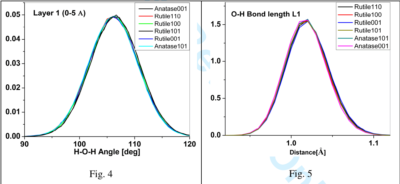
Fig. 4: Probability distribution of the water H-O-H angle in the adsorbed L1 (0-5 Å) in contact with each surface
