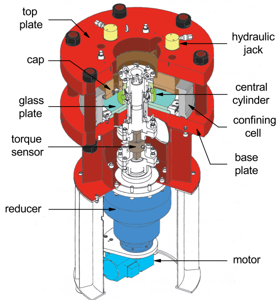
Fig. 19 Cut-away design view of ACSA.
