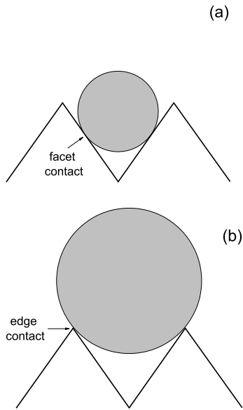
Fig. 3 Particle-wall contact for (a) d \leq d_{lim} and (b) d > d_{lim}
