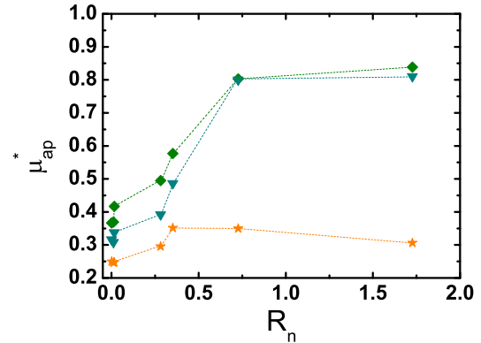
Fig. 9 Apparent effective coefficient of friction \mu_{\text{app}}^* for different reference points: ( \star ) 2, ( \nabla ) 3 or 3a and ( \blacklozenge ) 4.
