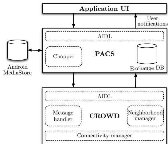
Figure 2: Extensible architecture of PePiT.
