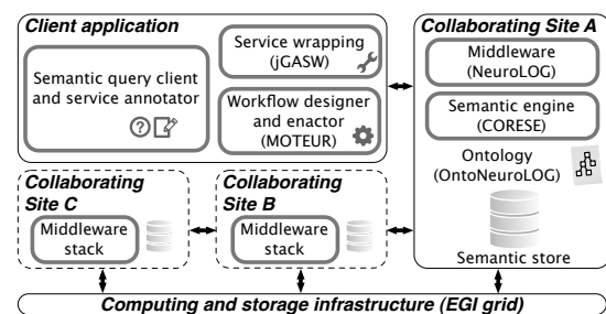
Figure 7: NeuroLOG platform: semantic enhancements to support the sharing and enactment of neuroimaging workflows.
