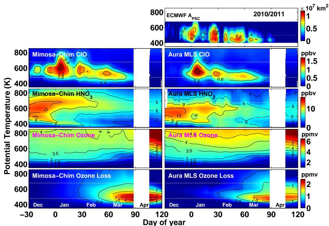
Fig. 5. Temporal evolution of the vertical distribution of CIO (second panel from the top), HNO 3 (third panel from the top), O 3 (fourth panel from the top), and ozone loss (bottom panel) from Mimosa-Chim and Aura MLS for the Arctic winter 2010/2011. The model fields are sampled at the location of MLS observations for each measurement inside the vortex and then averaged for the corresponding day. Both data are smoothed for seven days. The Model and MLS CIO coincident profiles are selected for solar zenith angles <89° and local time between 10 h and 16 h. The MLS CIO profiles are bias corrected (see text). The A PSC computed from the ECMWF operational analyses is also shown (top panel). The white dotted lines represent 475 K and 675 K. The blue/red colors show relatively low/high values of PSC areas or mixing ratios of CIO, HNO 3 , O 3 , and ozone loss.
