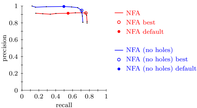
Fig. 23 NFA parameter tuning on the snow sequence. The performances of the two NFA algorithms (with holes and without holes) on the snow sequence are represented in the (recall,precision) plane in function of the threshold parameter \log_{10} \varepsilon . While the precision remains merely constant, a good recall is obtained with the default value (0) of \log_{10} \varepsilon , but the results can be improved by choosing a slightly greater value ( \log_{10} \varepsilon = +5 ), which corresponds for the two algorithms to the “NFA best” point.
