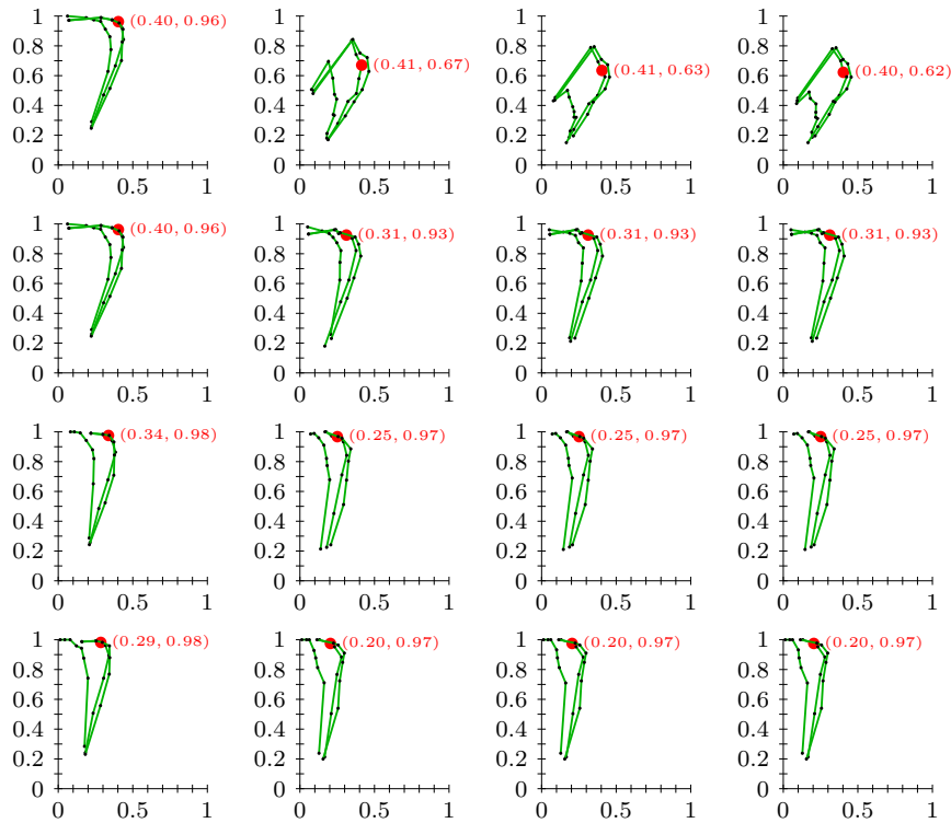
Fig. 22 ROADS parameter tuning on the snow sequence. We vary all ROADS parameters on the snow point sequence, and show the associated performances in the (recall,precision) plane using the available ground truth for that sequence. Each column has a distinct a_{\max} = 0, 4, 8, +\infty , and each row has a distinct p_{\min} = 1, 3, 5, 7 . Each curve corresponds to a different maximal smoothness criterion value \phi_{\max} = 0.2, 0.4, 0.6 and each point of a given curve corresponds to a different maximal speed criterion d_{\max} = 2, 5, 10, 15, 20, 25, 30, 40, 80 . The big red dot corresponds to the parameters \phi_{\max} = 0.4 and d_{\max} = 15 , which seem to achieve a good precision/recall compromise for all values of a_{\max} and p_{\min} . The numbers indicate the corresponding recall and precision.
