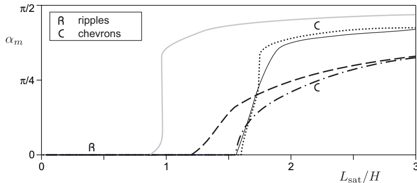
FIGURE 11. Pattern angle \alpha_m of the most unstable mode as a function of L_{\text{sat}}/H in the limit \mathcal{F} \rightarrow 0 . The grey solid line corresponds to the limit u_*/u_{\text{th}} \rightarrow \infty (for any value of \mu^{-1} ). The thin black solid line corresponds to the limit \mu^{-1} = 0 and u_*/u_{\text{th}} = 1 . The three other curves are computed with a finite avalanche slope \mu = \tan(32^\circ) , for u_*/u_{\text{th}} = 1 (dotted line), for u_*/u_{\text{th}} = 2 (dotted-dashed line) and for u_*/u_{\text{th}} = 4 (dashed line).
