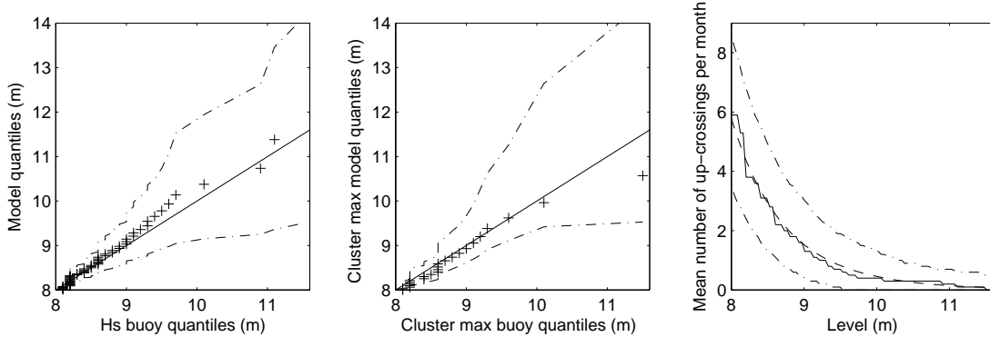
FIGURE 10. Comparison of the extremal behavior of the buoy data and fitted model. First panel: QQ-plot of the marginal distribution of the buoy ( x -axis) against the fitted model. Second panel: QQ-plot of the cluster maxima of the buoy ( x -axis) against the fitted model ( y -axis). Third panel: mean number of up-crossings per month as a function of the level ( x -axis) for the buoy data (solid line) and fitted model (dashed line). The dashed-dotted lines represent 95% prediction intervals computed by simulation (results based on 1000 independent replications of the fitted model simulated with the temporal sampling of the original data).
