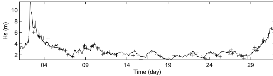
FIGURE 6. Comparison of the three time series for December 2005. Solid line: buoy data (location [47.5 N, 8.5 W]); dotted line: reanalysis data (location [48 N, 9 W]); plus points: closest satellite observation to the buoy from each satellite track within a 3° box.
