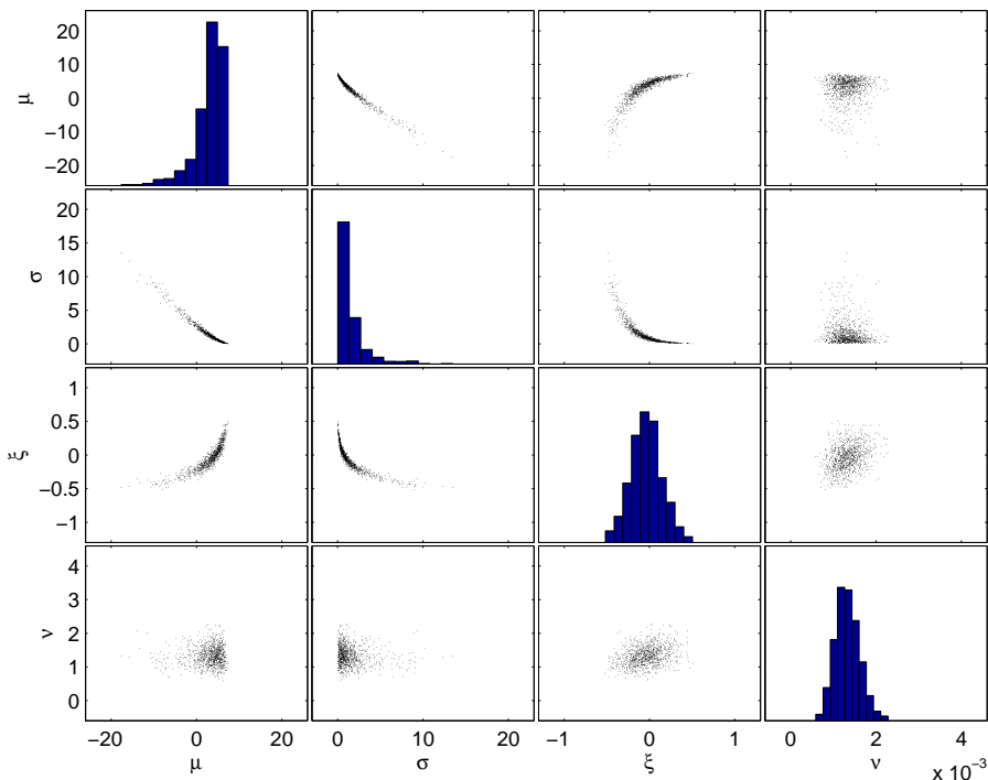
FIGURE 9. Empirical distribution of the parameters obtained using parametric bootstrap and the model fitted to buoy data. From left to right: estimates of \mu , \sigma , \xi , and \nu . The diagonal plots show histograms of the marginal distributions and the other plots are scatter plots of the bivariate distributions (results based on 1000 independent replications of the fitted model simulated with the temporal sampling of the original data).
