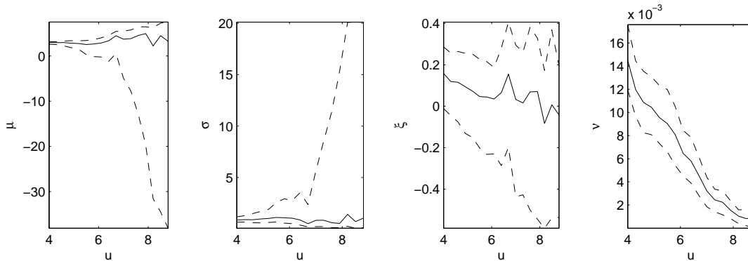
FIGURE 8. Values of the MPL_1E computed on buoy data as a function of threshold u ( x -axis). From left to right: estimates of \mu , \sigma , \xi , and \nu . The dashed lines correspond to 95% confidence intervals computed using parametric bootstrap (results based on 1000 independent replications of the fitted model simulated with the temporal sampling of the original data).
