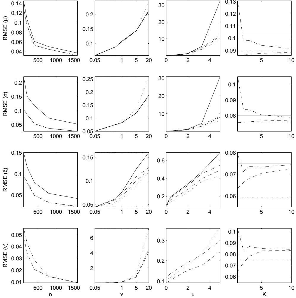
FIGURE 2. RMSE (y-axis) as a function of sample size n (first column), dependence parameter \nu (second column), threshold u (third column) and neighborhood size K (last column). Results obtained using 1000 simulations of a Gaussian extreme value process. Unless specified otherwise, the time sampling is regular and the values \mu = 0 , \sigma = 1 , \xi = 0.3 , \nu = 0.5 , u = -\infty , and n = 300 are used. Solid line: MILE; dotted line: MMLE; dashed line: MPL_1E ; dashed-dotted line: MPL_5E . For the last column, the time step between successive observations is drawn from a uniform distribution on the interval (0, 2) and the dashed [resp. dashed-dotted] line corresponds to the MPL_K E with the first [resp. second] weighting strategy (see (13) [resp. (14)]).
