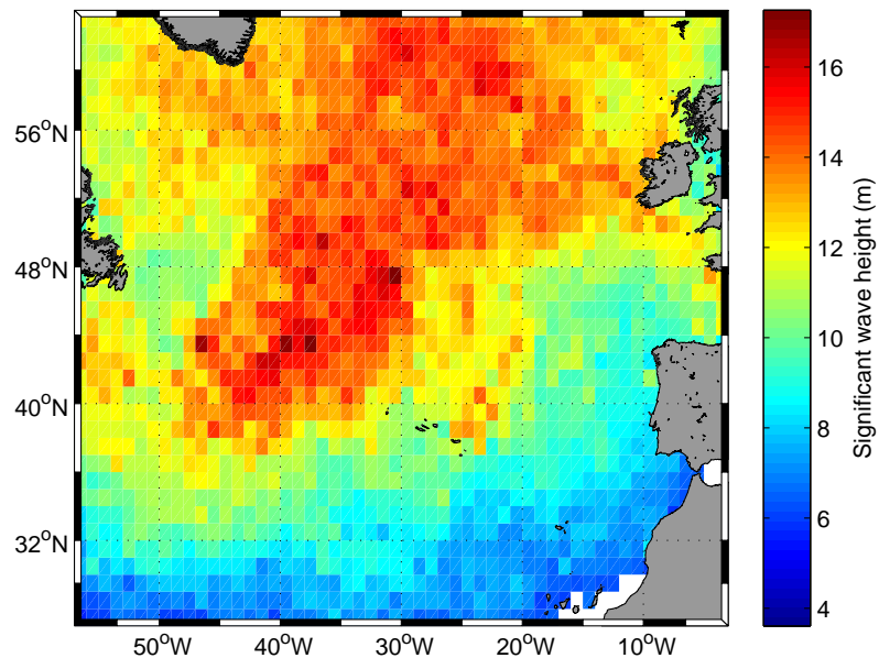
FIGURE 11. Map of 20-year return levels in the North Atlantic Ocean. A 3^\circ -wide moving window was used to build the time series at the different locations by retaining the value closest to the center for each satellite track crossing the window. A variable threshold corresponding to the 95% quantile was used.
