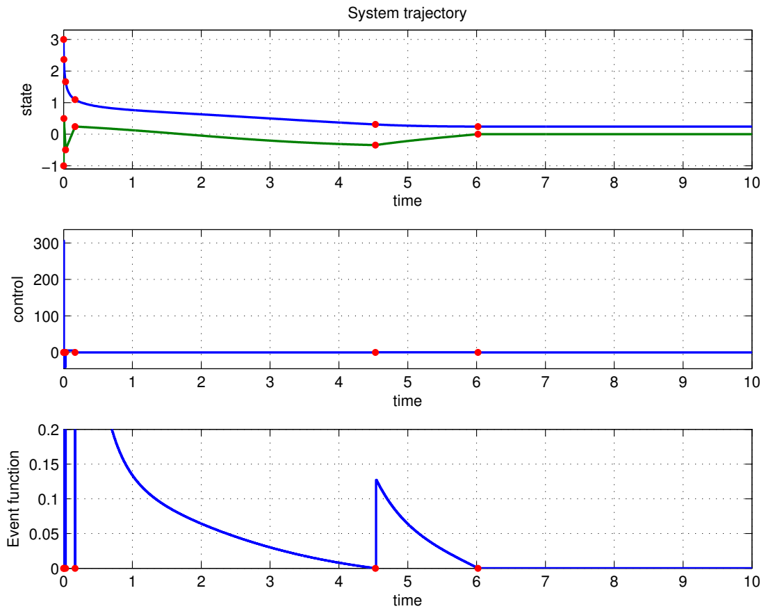
Figure 1: System (21) under event-based control with \alpha(x) = \beta(x) + a(x)^2 . The red dots represent the events instants.
