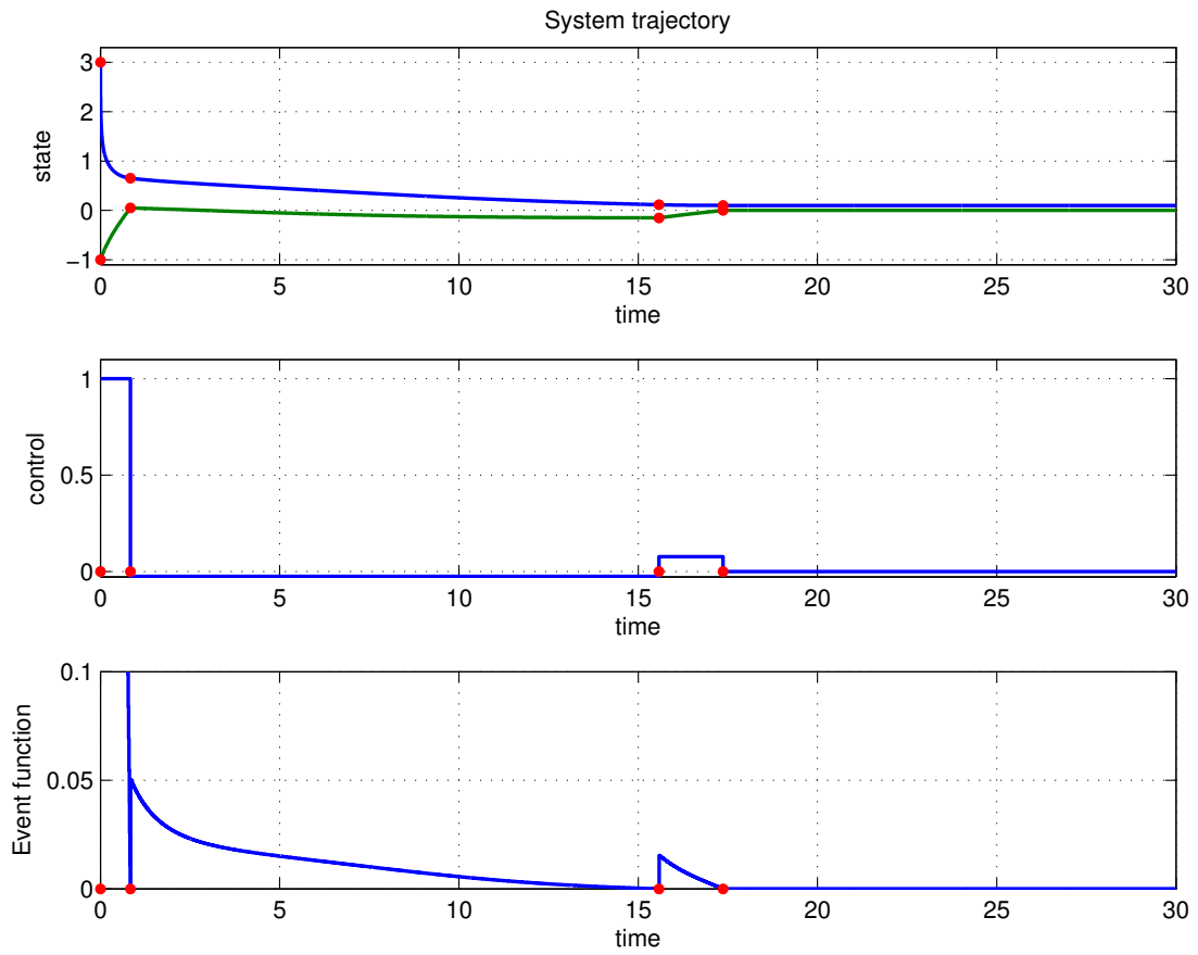
Figure 2: System (21) under smooth event-based control. The red dots represents the events instants.
