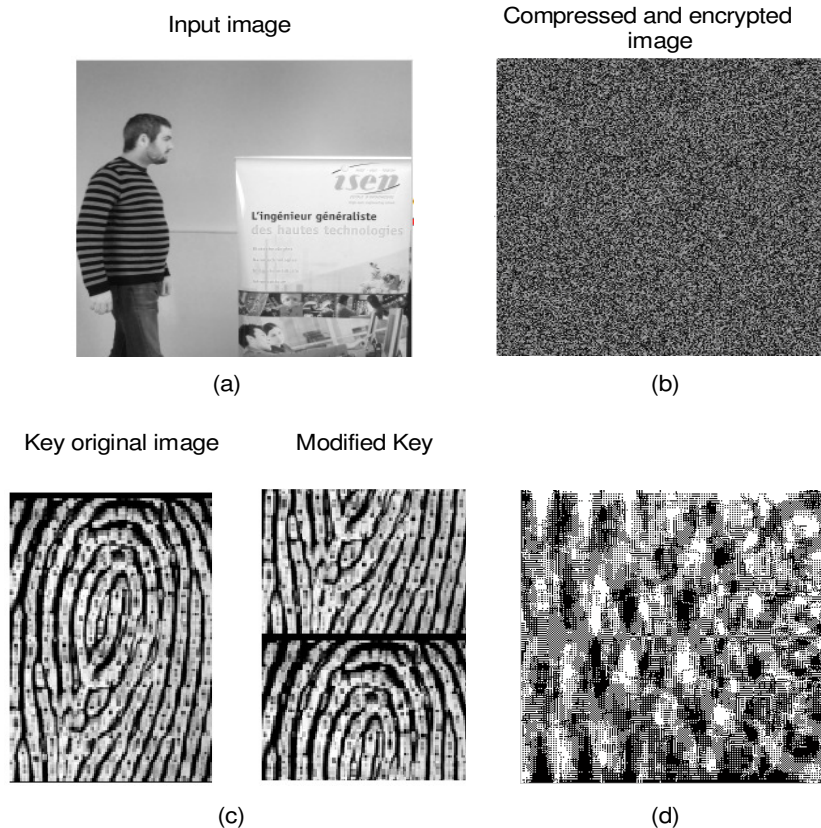
Fig. 4. Illustrating the three levels of encryption in our method: (a) the original target image, (b) the encrypted image with three levels of encryption (one of them is a fingerprint), (c) the modified fingerprint used for encryption of the second block of target images, and (d) simulation result when the cipher knows the principle of our method and when the access to the system is granted to him or her.
