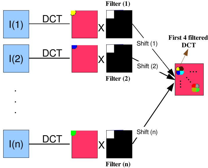
Fig. 1. Synoptic diagram illustrating the fusion method of multiple images, n is the number of target images. Rotation, shift, and 4 by 4 grouping constitute a first level of encryption.
