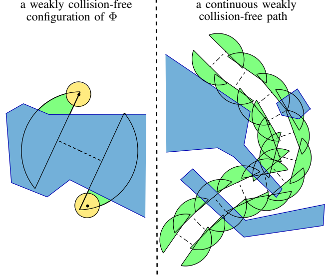
Fig. 5. Weak collision-freeness.
