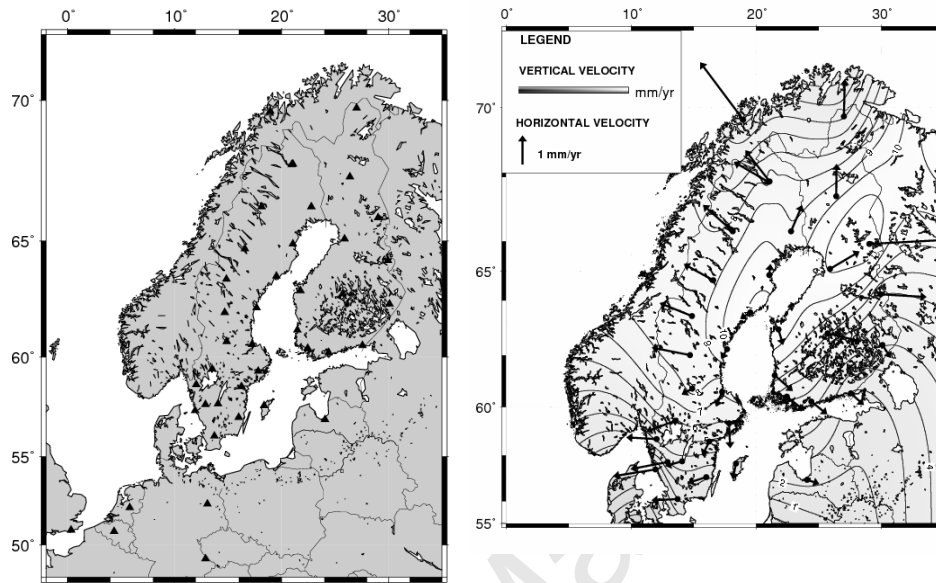
Figure 4: (Left) Data points used in the lithospheric thickness computation. (Right) Post-glacial rebound
