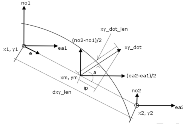
Figure 3: Graphical representation of the computation process.
