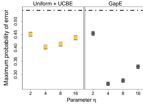
Figure 4: Problem 4: The benefit of adaptive allocation over the bandits in the twin bandits problem.
