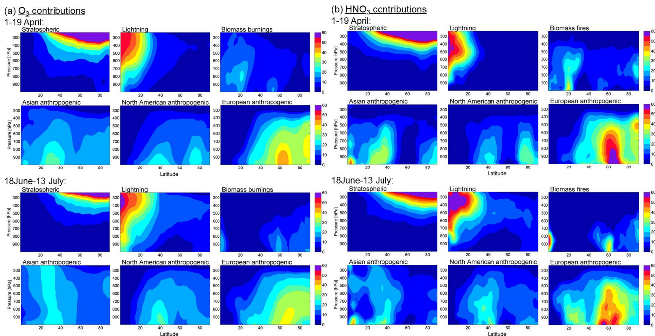
Fig. 10. Vertical and latitudinal distributions of the relative contributions (%) to \text{O}_3 (a) and \text{HNO}_3 (b) concentrations during the spring (from 1 to 19 April) and summer (from 18 June to 13 July) ARCTAS campaigns, as simulated by MOZART-4.
