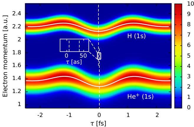
Figure 1. Streaking spectrograms for an 800 nm IR laser field with a duration of 3 fs and an intensity of 10^{12} W/cm ^2 . The graphs show the final momentum distribution in “forward” direction of the laser polarization axis for H(1s) and He ^+ (1s) initial states and an XUV photon energy of 80 eV. The solid white lines are the first moments of the electron spectra. The dashed white vertical lines indicate the shift of the central minimum relative to the vector potential. The colour scale is in arbitrary units.
