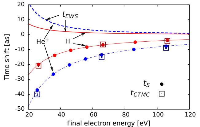
Figure 2. Temporal shifts t_S extracted from quantum mechanical streaking simulations (H(1s): red circles, He ^+ (1s): blue circles), classical streaking simulations (H(1s): red squares, He ^+ (1s): blue squares), and for comparison, the EWS time shift t_{\text{EWS}} = d\varphi/dE applied to the Coulomb phase (H ^+ : red solid line, He ^{2+} : blue dashed line).
