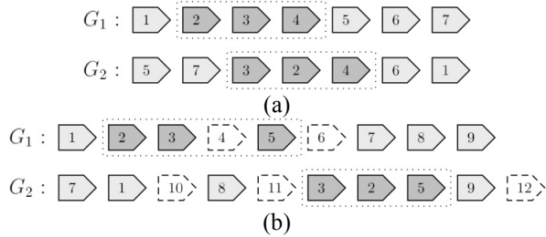
Figure 1. Illustration of a common interval between genomes G_1 and G_2 . The set of genes \{2, 3, 4\} is a common interval since genes 2, 3 and 4 are consecutive in both genomes. (b) Illustration of a common interval between two genomes which do not have the same gene contents. The set of genes \{2, 3, 5\} is also a common interval since genes 2, 3 and 5 are consecutive in both genomes, when we consider only genes that are present in both genomes (genes 1, 2, 3, 5, 7, 8 and 9). Dashed genes (4, 6, 10, 11, 12) are left aside before common intervals computation since they are not present on both genomes. After intervals computation, these genes are then re-introduced into common intervals.
