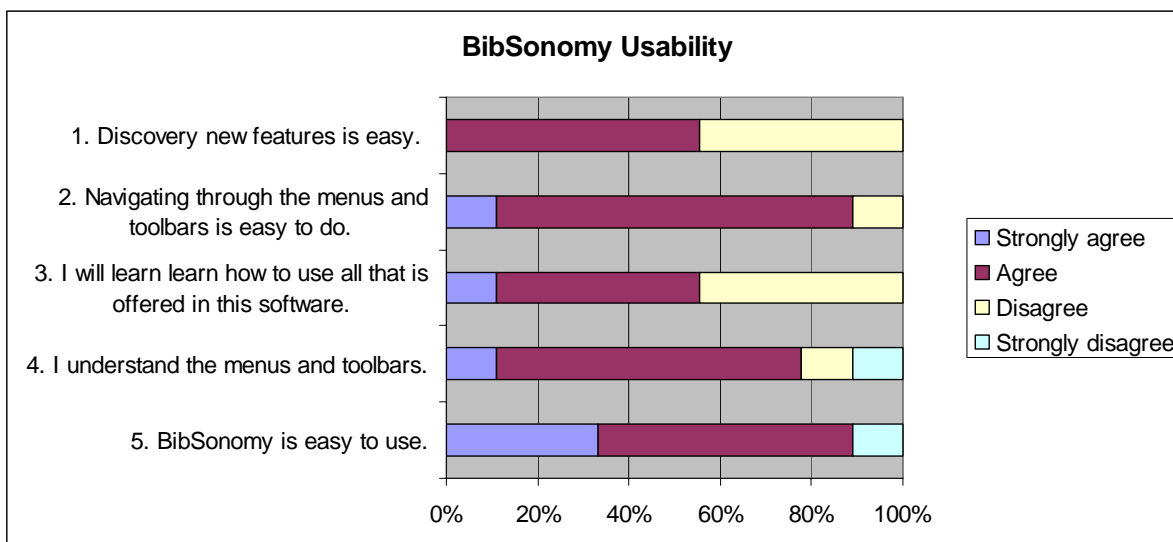
Figure 11: BibSonomy Usability
