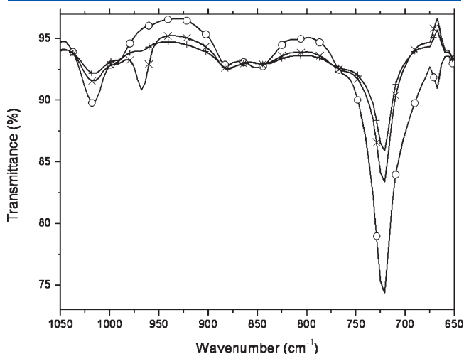
Figure 2. Infrared spectra for the photoreaction of a 3/1 dodecane-thiol/methyl oleate mixture: infrared spectrum after 0 (O), 5 (×), and 60 min (+) of reaction. A UV irradiance of 15 W/cm 2 was used.
