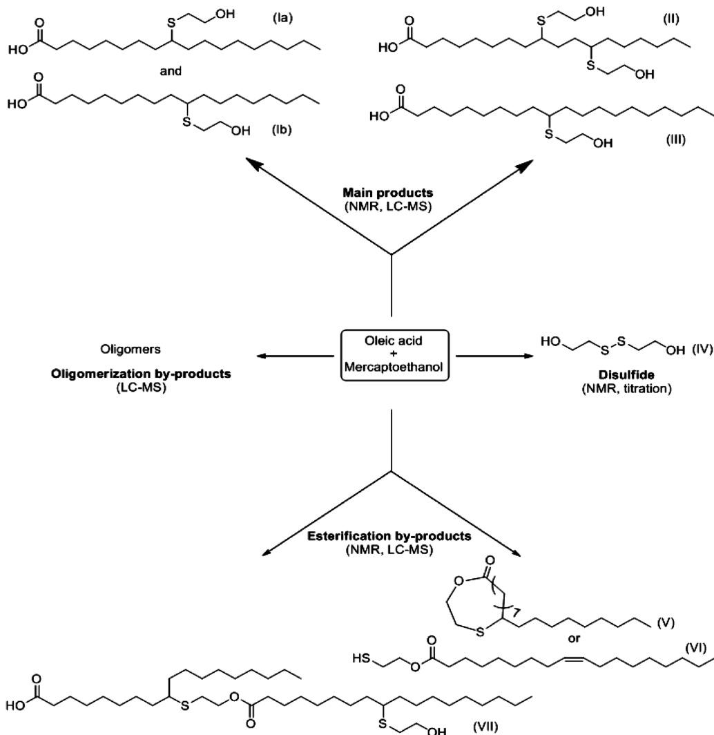
Figure 4. Expected products and byproducts obtained by thiol–ene photoaddition of mercaptoethanol onto oleic acid and their identification techniques.
