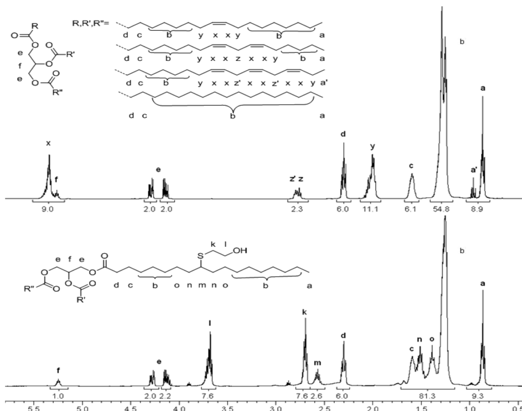
Figure 7. ^1\text{H} NMR spectra ( \text{CDCl}_3 ) of rapeseed oil and its product after the thiol–ene coupling with 2-mercaptoethanol. A thiol/double bond ratio of 3/1 was irradiated 5 h at 15\text{ W/cm}^2 .
