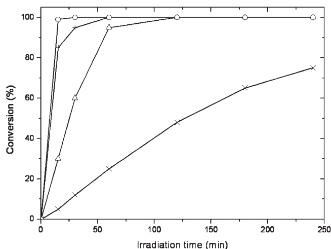
Figure 5. Double-bond conversion during the photoaddition reaction of 2-mercaptoethanol onto oleic acid irradiated at 15 W/cm 2 at different thiol/ene ratio: 1.2/1 (x), 2.0/1 (Δ), 3.0/1 (+), and 5.0/1 (O).
