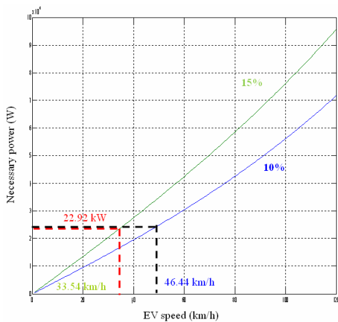
Fig. 6. The induction motor necessary power for gradeability.
