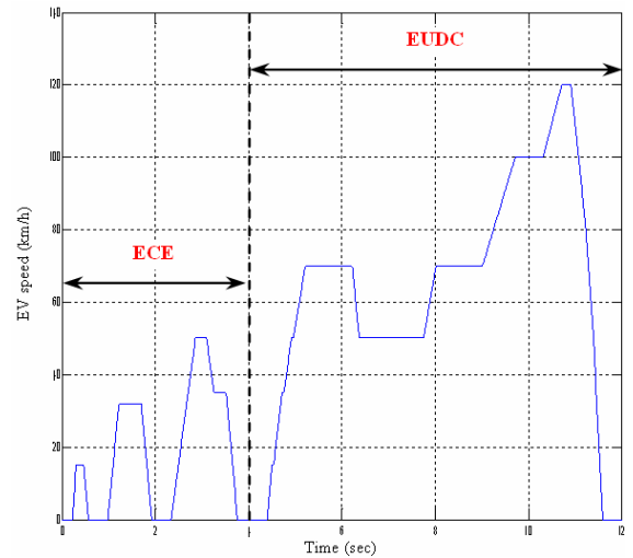
Fig. 7. The European ECE + EUDC driving cycle.
