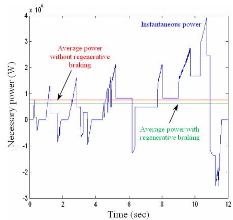
Fig. 8. The induction motor necessary power for the ECE + EUDC driving cycle.
