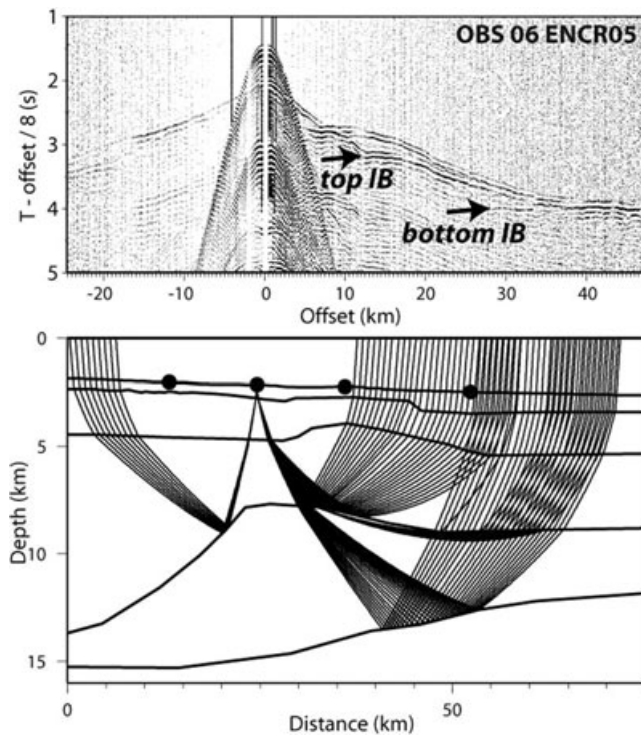
Figure 12. Upper panel: OBS 06 record section on ENCR05 shot line. IB: intermediate velocity body reflections. Lower panel: Ray tracing diagram for top of the intermediate body reflections, refractions in the intermediate body and reflections on the base of the intermediate body.
