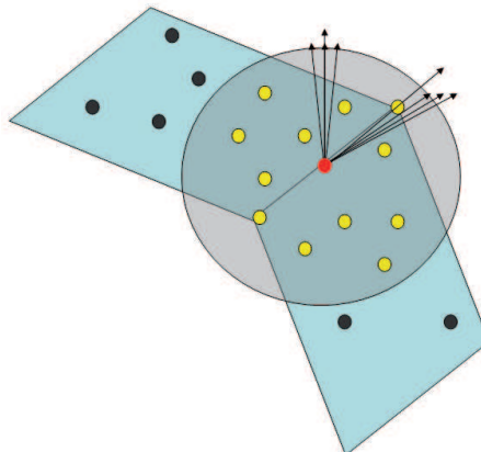
Fig. 1. Computation of the normal vectors used for feature identification in a local neighborhood.
