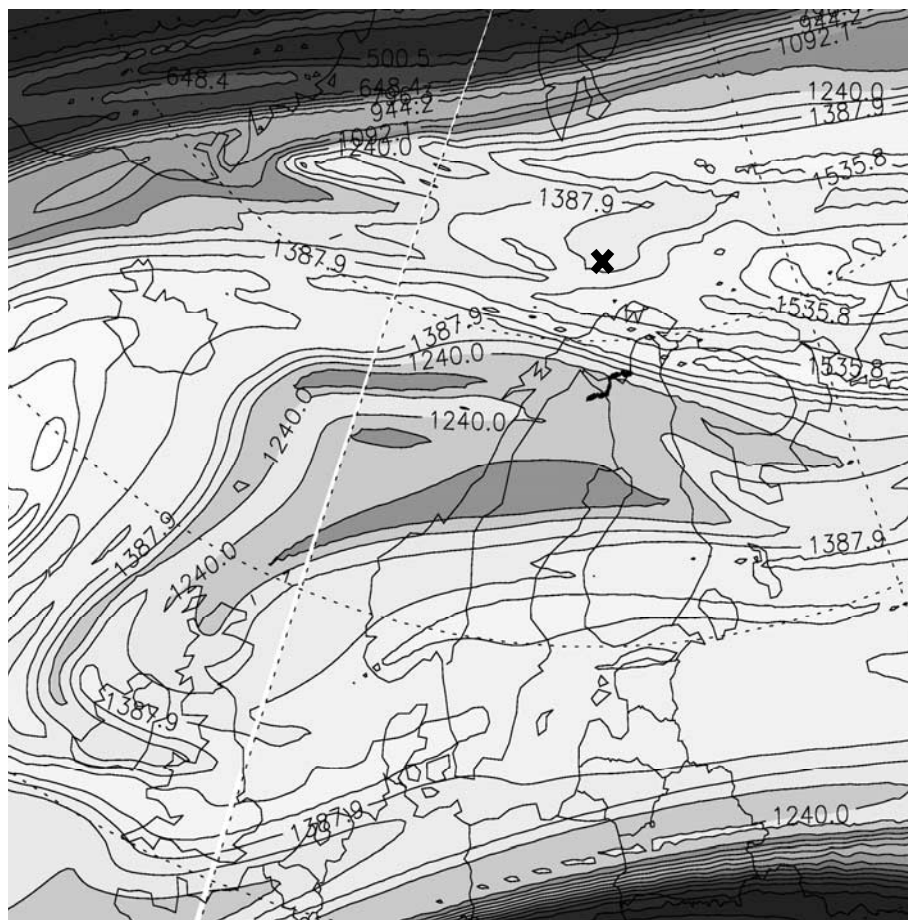
Figure 5. Potential Vorticity isocontours in pvu ( 1 \text{ pvu} = 10^{-6} \text{ m}^2 \text{ s}^{-1} \text{ kg}^{-1} \text{ K} ) calculated by the MIMOSA high-resolution model at 950 K (about 32 km) on 16 January 2006 at 1800 UT. The positions where the lines of sight of SALOMON intersect this level are also shown (bold black line above Scandinavia). GOMOS measurement positions are also shown (thick cross).
