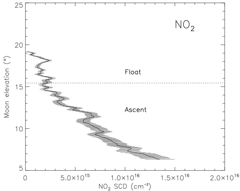
Figure 7. NO 2 SCDs measured by SALOMON for varying moon elevation angles during the balloon ascent and at float altitude (about 33 km). Note that the SCD value at 19.5° corresponds to the spectrum used as reference.
