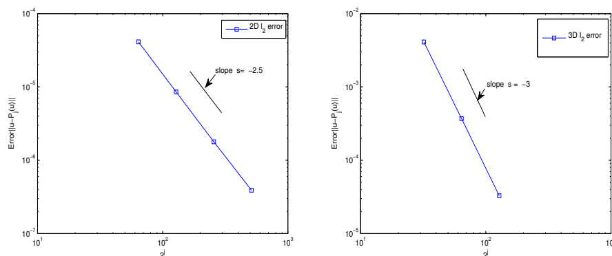
Figure 7. \ell_2 -projection error onto \mathbf{V}_j^{div} versus j . Two-dimensional case (left) and three-dimensional case (right). The generators (\varphi^1, \tilde{\varphi}^1) correspond to biorthogonal splines with r = \tilde{r} = 3 .
