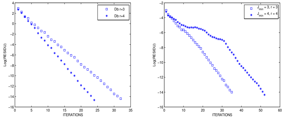
Figure 3. Preconditioned conjugate gradient residuals versus iteration number, for different values of the approximation order r : periodic case (left) and non periodic case (right). Daubechies generators \psi^1 with r = 3 and r = 4 vanishing moments. The resolution is j = 10 in two dimension ( d = 2 ).
