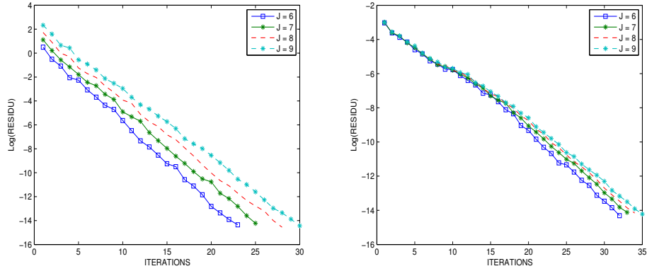
Figure 2. Preconditioned conjugate gradient residual versus iteration number, for different values of the dimension index j : periodic case (left) and non periodic case (right). Daubechies generators \psi^1 with r = 3 vanishing moments, j_{min} = 3 in non periodic (2D case).
