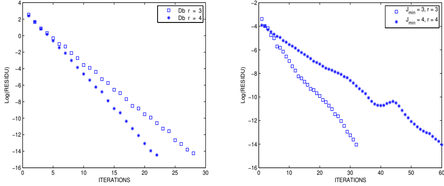
Figure 4. Preconditioned conjugate gradient residuals versus iteration number, for different values of the approximation order r : periodic case (left) and non periodic case (right). Daubechies generators \psi^1 with r = 3 and r = 4 vanishing moments. The resolution is j = 7 in three dimension ( d = 3 ).
