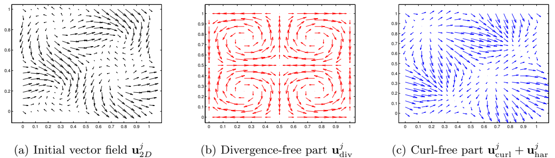
Figure 5. Example of Helmholtz decomposition.
