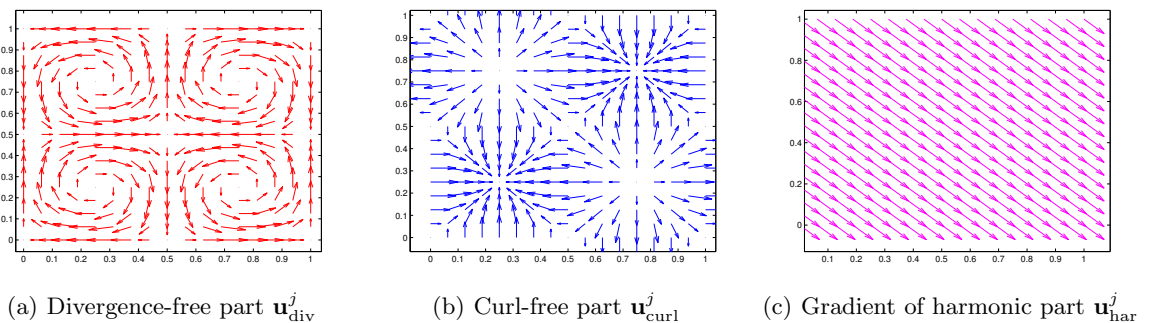
Figure 6. Example of Helmholtz-Hodge decomposition.
