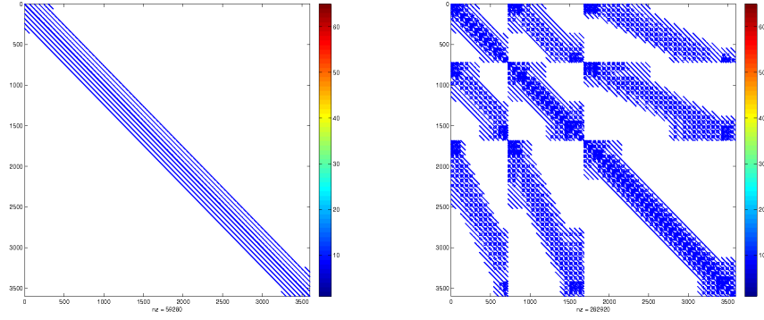
Figure 1. Gram matrices of divergence-free scaling functions (left) and wavelets (right) built from Daubechies generators with r = 3 , j_{min} = 4 , j = 6 .
