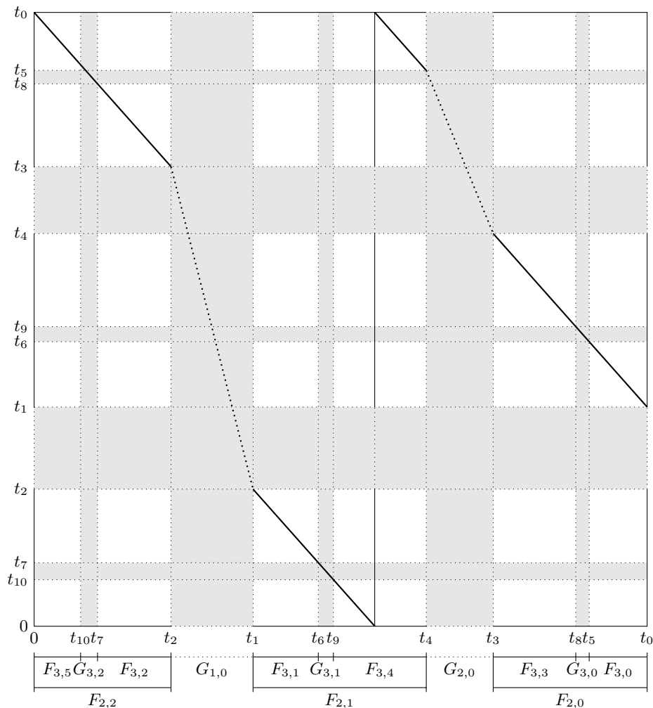
FIGURE 3. The (-\beta) -transformation for \beta = 9/8 with gaps G_{m,k} , support of the invariant measure F_{3,0} \cup \dots \cup F_{3,5} , and t_k = T^k_{-\beta}(1) . Ratios between G_{1,0} , G_{2,0} and the rest of the picture are not respected. In reality, G_{1,0} is almost 10 times the size of G_{2,0} , and G_{2,0} is almost 5 times the size of F_{2,0} .
