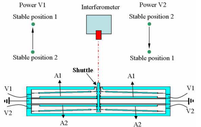
Fig. 8. Switching test using a high resolution interferometer.
