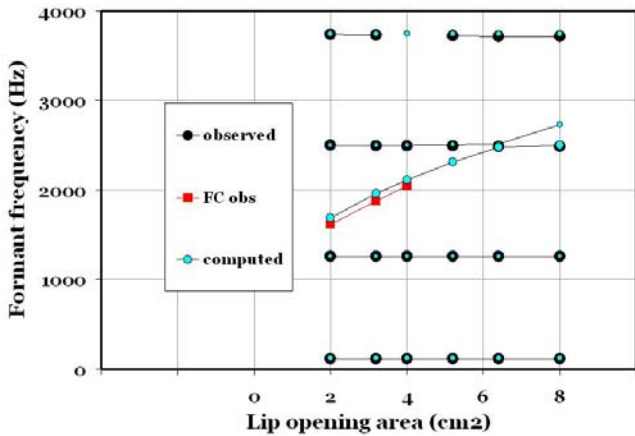
Figure 10. Formant frequencies plotted against lip opening area for an empty subapical cavity and varying lip aperture. Measured F1 F2 F4 and F5: solid black circles. Computed (all formants): light blue circles. The measured F3 (front cavity): solid red squares.
