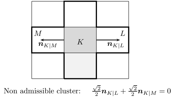
FIGURE 2. Admissible and non admissible clusters. For a given cell K (in dark gray), the set of cells defining the cluster G_K is colored in gray (and includes K ), and the set \mathcal{N}_K of neighbouring cells to K is outlined with a bold line.
