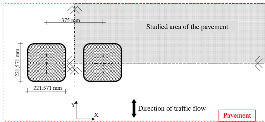
Figure 1: Tire contact area of the dual-axle traffic load
