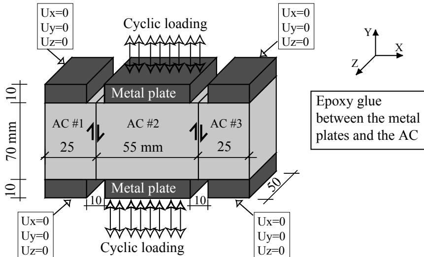
Fig. 1. Schematic diagram of the double shear test
