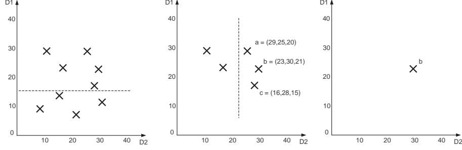
Figure 1. A set of vectors in a three dimensional space D1 \times D2 \times D3 , and the three iterations of the \alpha -trimmed lexicographical maximum computation with \alpha = 0.5 (left to right). According to the proposed approach, the maximum will be the greatest, with respect to the third dimension, of the remaining three vectors.
