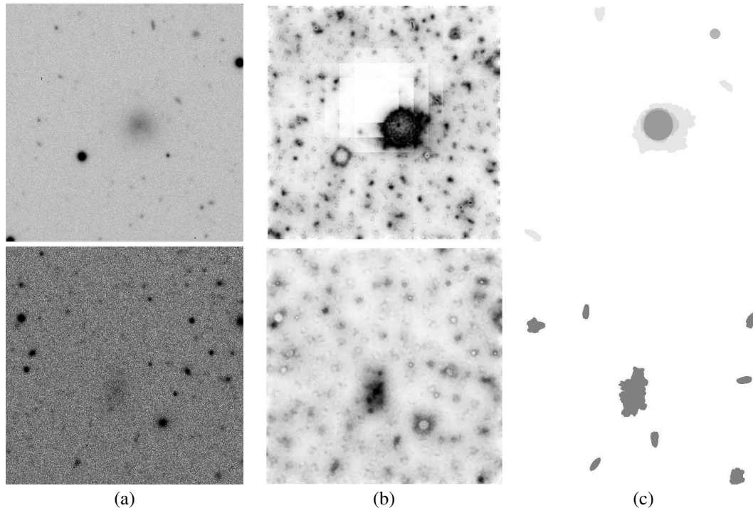
Figure 5: Application of FHMT to LSB detection, easy (top) and hard (bottom) cases. From left to right: contrast-stretched view of the original image of 512 \times 512 pixels with an LSB galaxy at center, score map obtained after application of FHMT, and final map containing different classes proportional to the object luminosity allowing deblending capabilities for overlapping object having different luminosities.
