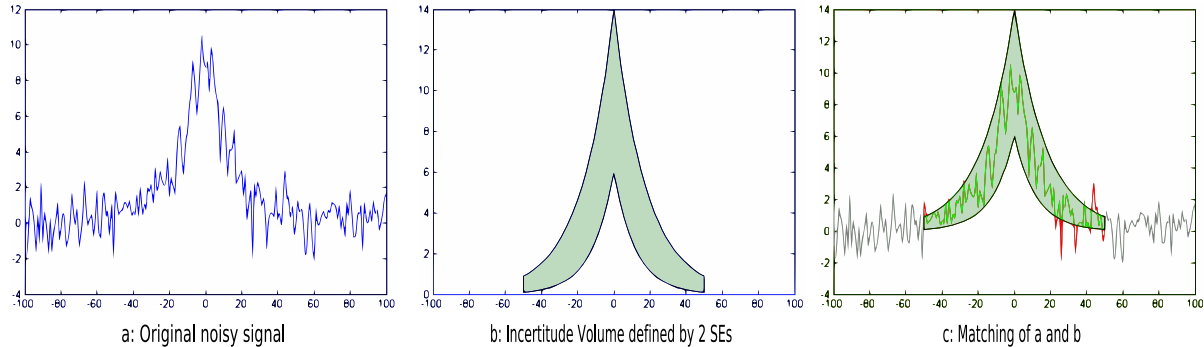
Figure 2: Example of application of the fuzzy hit-or-miss transform to detect an exponential profile with gaussian noise. Image (a) represents a 1D noisy signal ( \text{SNR} \approx 9\text{dB} ). Image (b) represents the incertitude area defined by the 2 SEs F and B . Image (c) shows how well the pattern can fit the signal.
