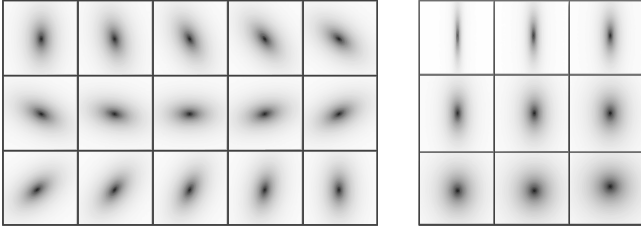
Figure 4: Example of SEs obtained with a variation of orientation (left) and of elongation (right) convolved with a gaussian point spread function.
