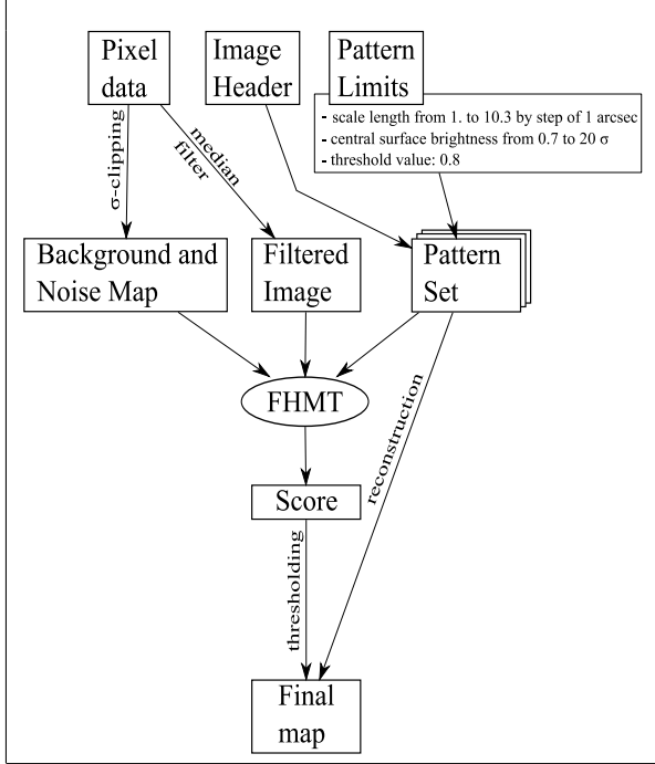
Figure 3: Scheme of the LSB galaxy detection method. The algorithm takes three inputs: image pixels values, image header, and pattern limits (based on physical criteria.) The whole procedure is automatic.
