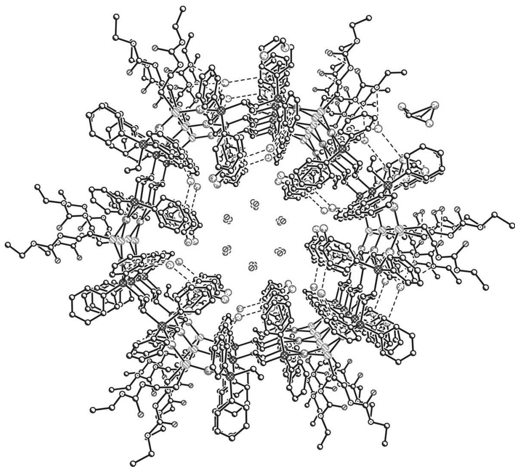
Figure 4. View along the c-axis of the helical arrangement observed in the crystal packing of 11. The assembly gives rise to channels inside of which water molecules are found. 202x182mm (150 x 150 DPI)
