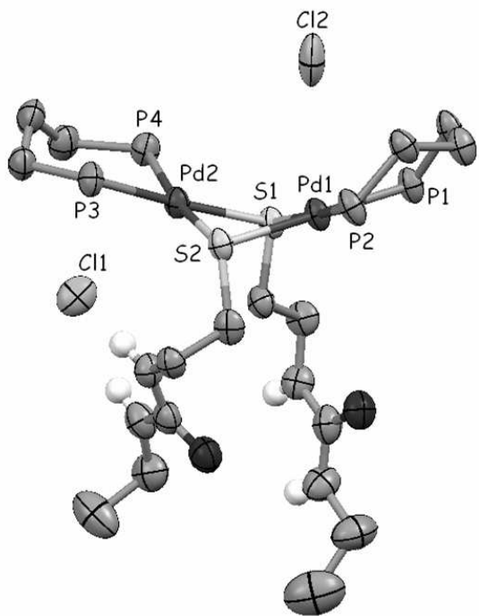
Figure 3. Ortep-Plot (thermal ellipsoids shown at 50 % probability level) of 11. Phenyl rings of the dppp ligands and the molecule's hydrogen atoms (except those of the urea groups) have been omitted for clarity. 254x190mm (96 x 96 DPI)
