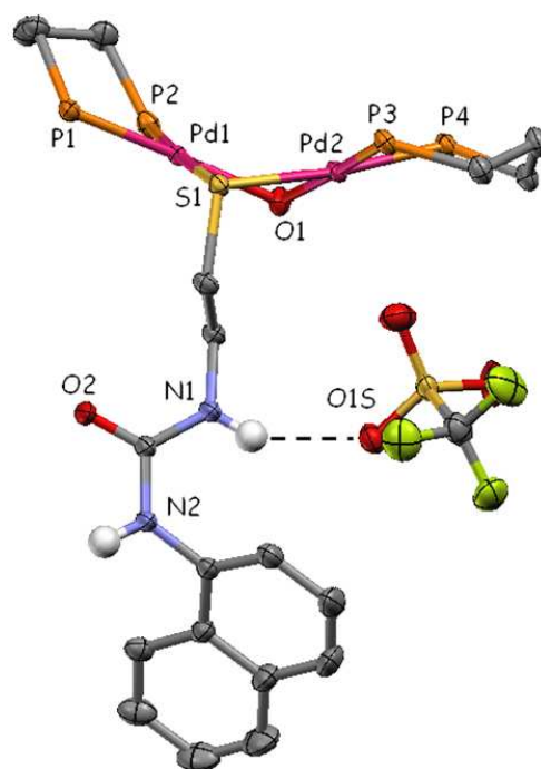
Figure 9. Ortep-Plot (thermal ellipsoids shown at 50 % probability level) of 12. Phenyl rings of the dppp ligands and the molecule's hydrogen atoms (except those of the urea groups) have been omitted for clarity. 254x190mm (96 x 96 DPI)
