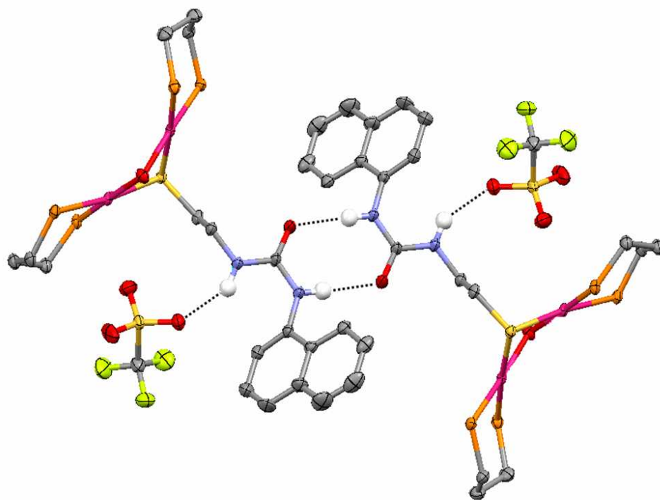
Figure 10. Molecular structure showing the dimer of 12 observed in the crystal packing. Distance of the symmetric hydrogen bonds: O2 \cdots N2A: 2.973(2) Å. Phenyl rings of the dppp ligands and the molecule's hydrogen atoms (except those of the urea groups) have been omitted for clarity.
