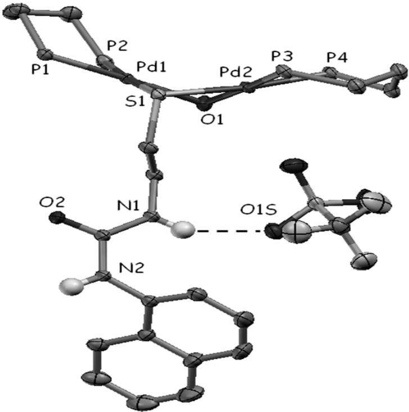
Figure 9. Ortep-Plot (thermal ellipsoids shown at 50 % probability level) of 12. Phenyl rings of the dppp ligands and the molecule's hydrogen atoms (except those of the urea groups) have been omitted for clarity. 150x182mm (150 x 107 DPI)
