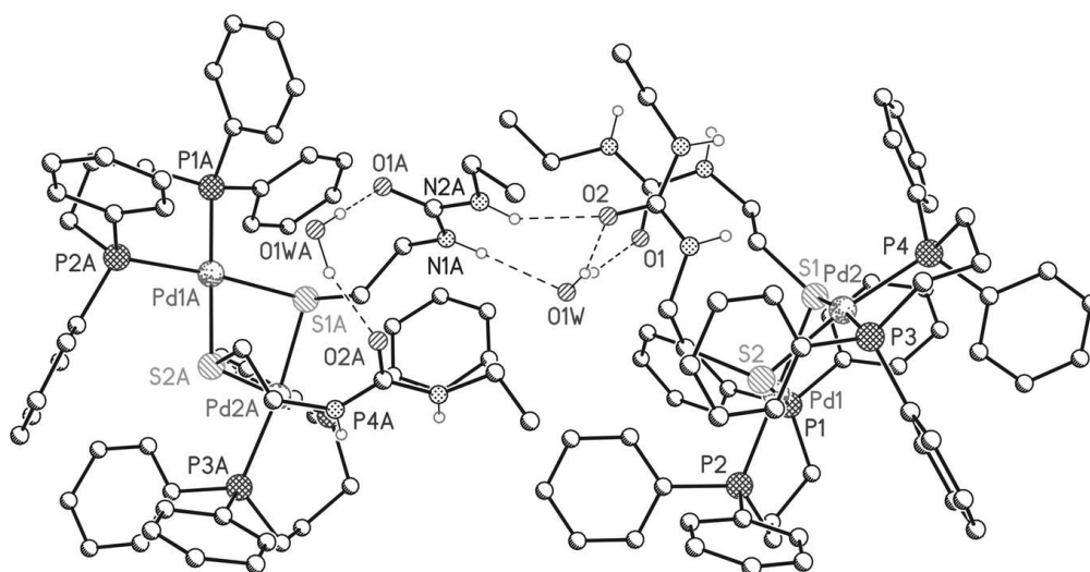
Figure 5. Molecular structure showing the hydrogen bonds between the urea groups and a water molecule. Distances: O1W...O1: 2.773(3) Å; O1W...O2: 2.781(3) Å; O1W...N1A: 3.038(4) Å; N2A...O2: 2.893(4) Å.
