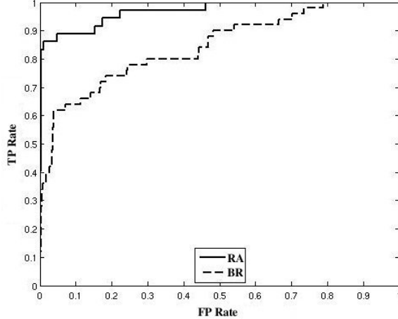
Fig. 8. The ROC curves associated to the classification by the SMC_{\mathcal{R}_A} and the SMC_{\mathcal{B}\mathcal{R}} classifiers.
