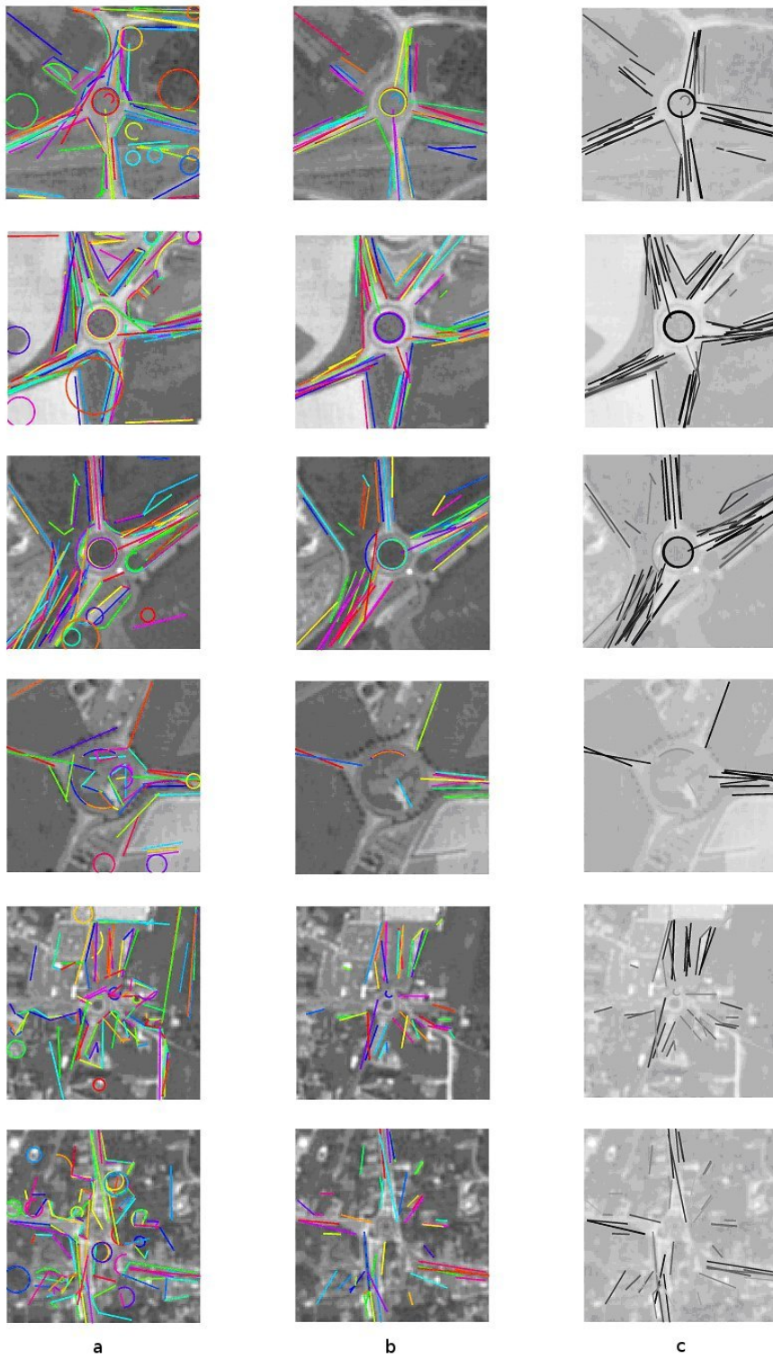
Fig. 9. The 3 best ranked, and the 3 worst ranked roundabout images in SMC_{RA} , (a). All detected primitives, (b). Selected primitives, (c). represented by a gray level corresponding to their membership score.
