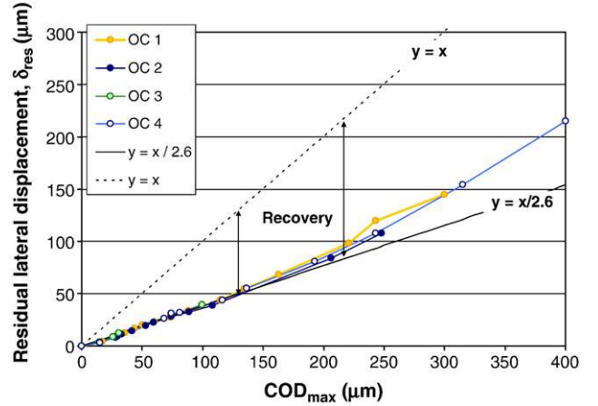
Fig. 8. COD recovery after unloading of OC.
