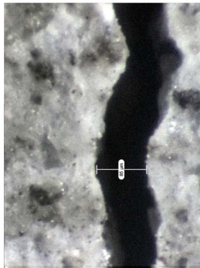
d) \text{COD}_{\text{max}} = 215 \text{ } \mu\text{m} , w_1 \approx 85 \text{ } \mu\text{m}
